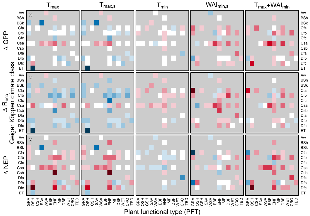
Figure 7: Z-transformed flux differences Differences between z-transformed \text{CO}_2 fluxes during extreme events and reference periods for the different extreme event types and the different fluxes ( \Delta z = z_{extr} - z_{ref} , see Eq. 2 and 3 for details) of the different extreme event types on GPP, R_{eco} and NEP (rows 1 - 3) separated according to plant functional types (PFT) (x axis in each plot, Tab. 2 for the acronyms used) and Geiger Köppen climate class (y axis in each plot, Tab. 3 for the acronyms used) for different types of extreme events (columns 1- 5: heat ( T_{max} ), heat alone ( T_{max,s} ), cold ( T_{min,s} ), drought alone ( WAI_{min,s} ) and combined heat and drought ( T_{max}+WAI_{min} )). Shades of red indicate reductions of different size in the respective fluxes, shades of blue increases. Refer to figures 5 and 6 for a visualization or quantification of the actual magnitude of these impacts.
