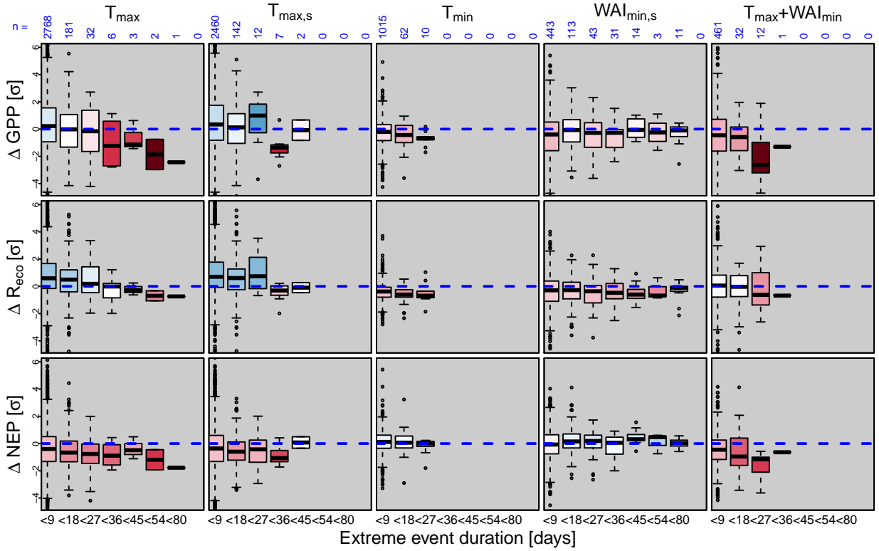
Figure 4: Influence of extreme event duration on extreme event impact. Shown are normalized flux differences between extreme events and a reference period ( \Delta z = z_{extr} - z_{ref} , see Eq. 2 and 3 for details) for gross primary production (GPP), ecosystem respiration ( R_{eco} ) and net ecosystem production (NEP) (in rows 1 - 3) for a selection of different extreme event types (in columns 1 - 5: heat ( T_{max} ), heat only ( T_{max,s} ), cold ( T_{min} ), drought only ( WAI_{min,s} ) and combined drought and heat ( T_{max}+WAI_{min} ), Tab. 1 for details on all extreme types).
