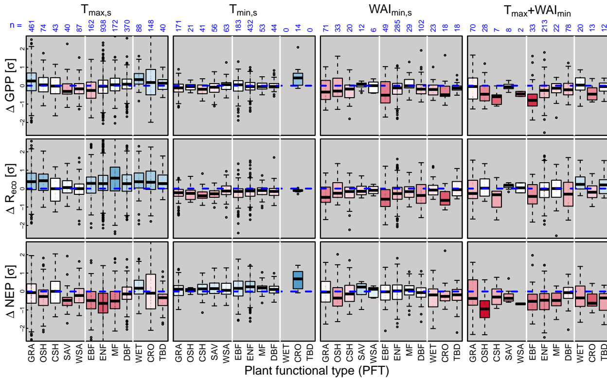
Figure 5. Differences between z-transformed \text{CO}_2 fluxes during extreme events and reference periods for the different extreme event types and the different fluxes ( \Delta z = z_{extr} - z_{ref} , cf. Eq. 2 and 3 for details) according to the Plant Functional Type (PFT) (Tab. A1 for the acronyms used) of the respective ecosystem (Fig. 6 for a detailed description of the boxplots shown).
