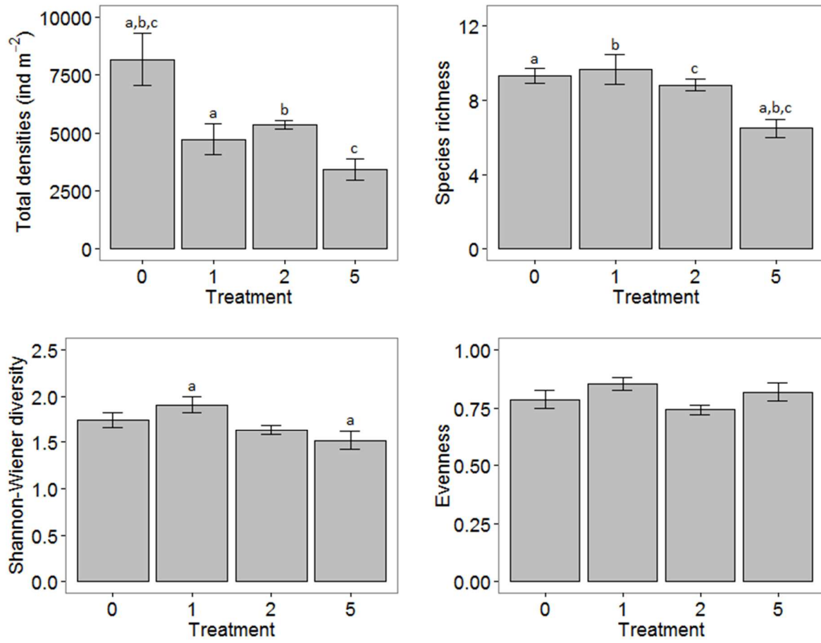
Figure 1: Bar charts representing total macrofaunal densities (ind m -2 ), species richness, Shannon-Wiener diversity, and Pielou's evenness per treatment. Error bars represent mean \pm standard error, letters above the error bars indicate pair-wise significant differences. The four treatments represent the thickness of the applied sediment layer (in cm).
