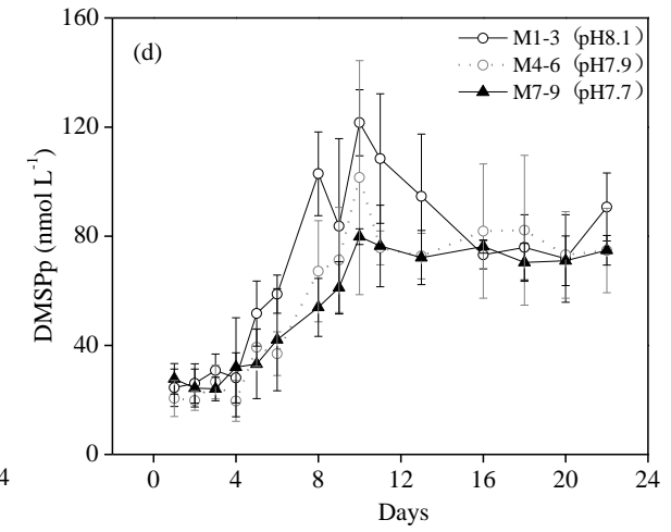
3 Figure 5. Temporal changes in the DMSPd and DMSPp concentrations ( \text{nmol L}^{-1} ) for (a, c) each of the nine barrels and (b, d)
