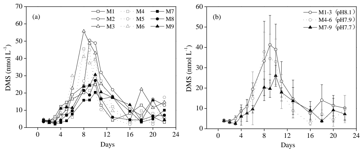
1 2 Figure 4. Temporal changes in the DMS concentrations (nmol L -1 ) for (a) each of the nine barrels and (b) averages over the 3 triplicates treatments.
