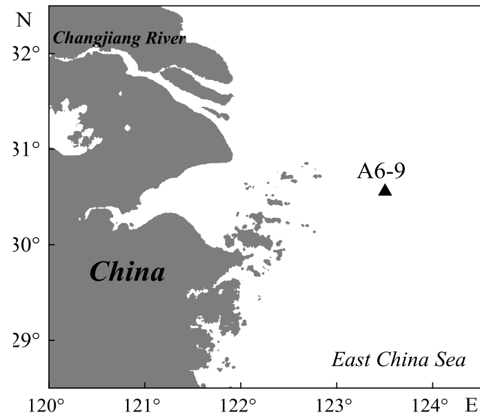
Figure 1. Location of the sampling station (123.50 °E, 30.56 °N) during the cruise.
