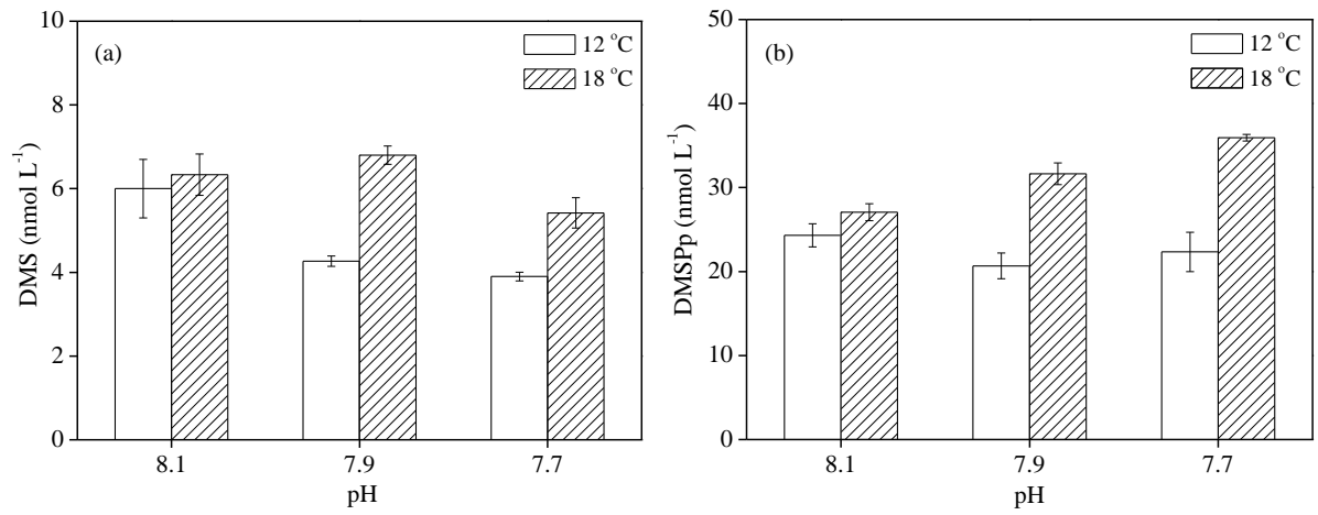
1 2 Figure 7. Average values of (a) DMS and (b) DMSPP concentrations in the cross experiment of OA and temperature, with 3 three replicate incubation samples per treatment.
