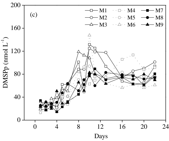
3 Figure 5. Temporal changes in the DMSPd and DMSPp concentrations ( \text{nmol L}^{-1} ) for (a, c) each of the nine barrels and (b, d)
