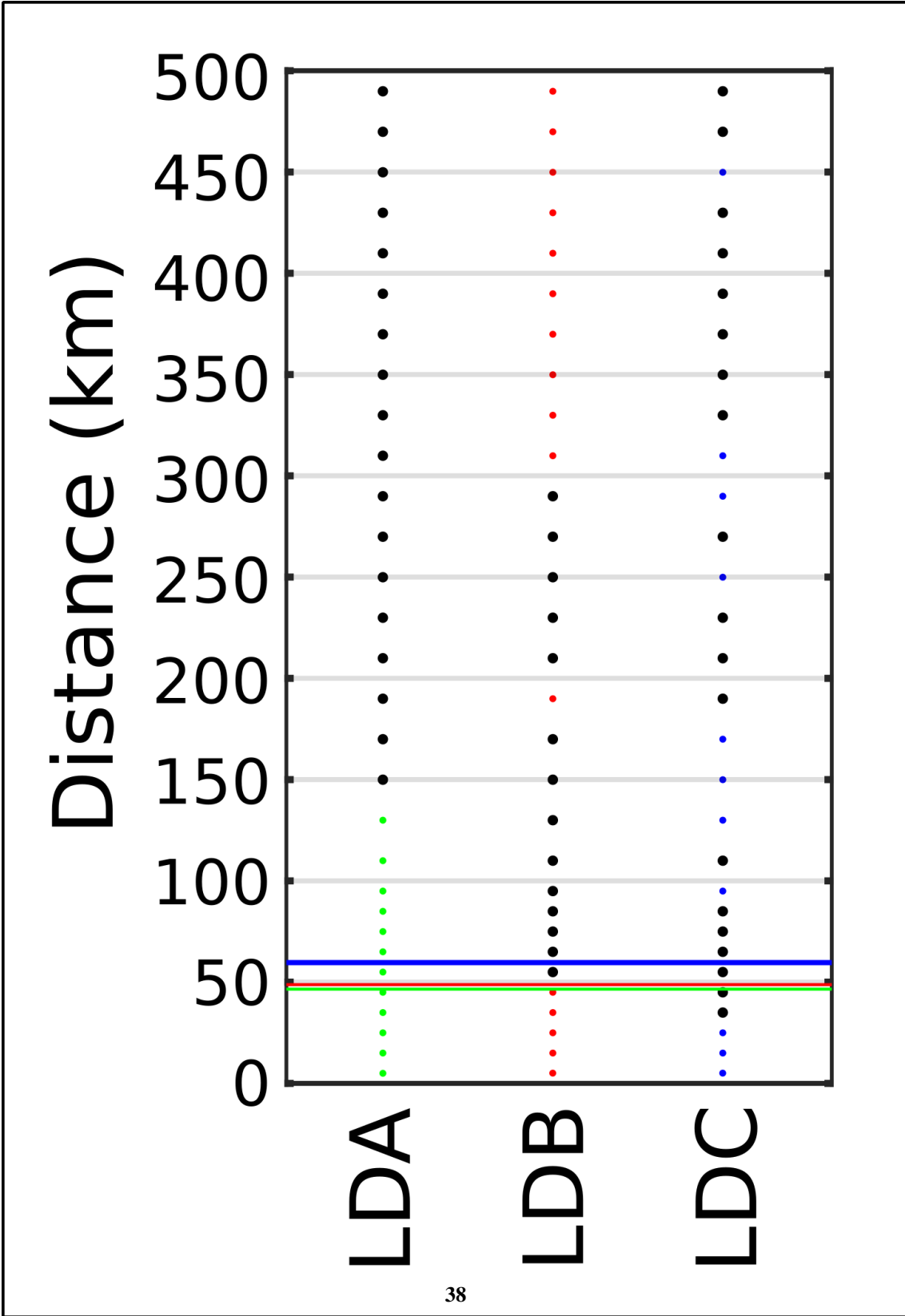
Figure 12. TSG Z-score over distance for LDA( left, green), LDB (center, red), and LDC (right, blue). |Z| > 2 shaded black. Rossby radii R_D
