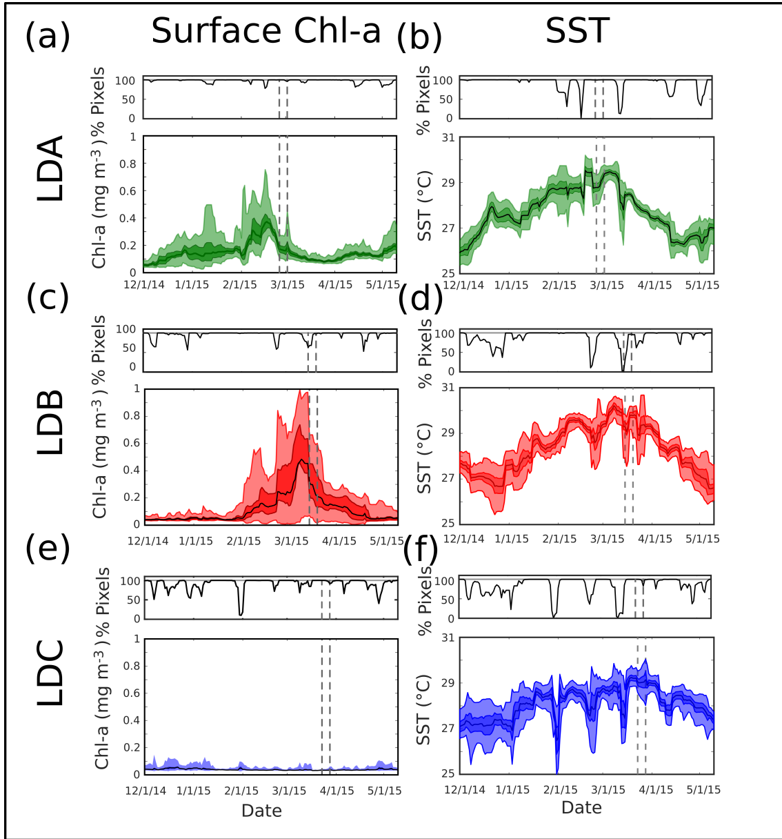
Figure 3. Timeseries of surface chl- a and SST, respectively, for (a,b) LDA, (c,d) LDB, and (e,f) LDC. Intervals of LD sampling shown with gray dashed lines. Mean values are plotted in black, with darker shades representing the 25-75% interval and lighter shades for 1-99%. Subpanels above each timeseries depict the % of pixels with data. All data come from within the 120 km \times 120 km squares shown in Fig. 2.
