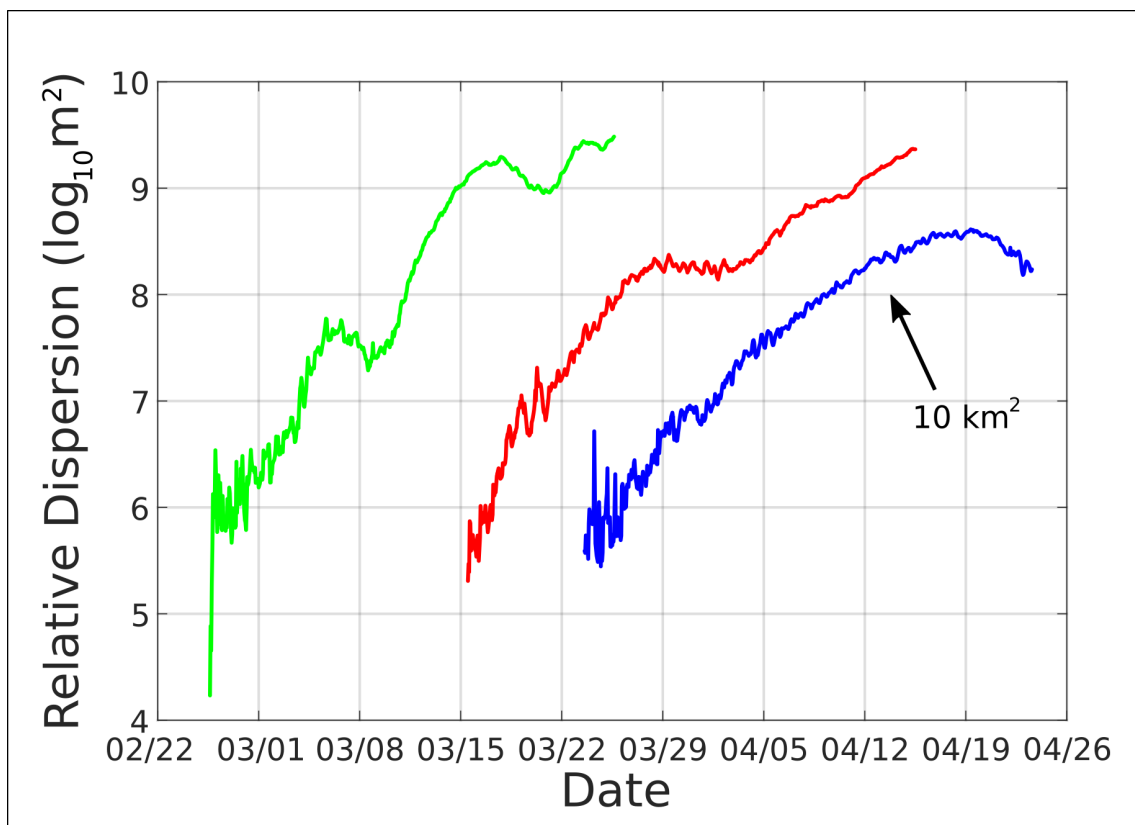
Figure 17. Supplementary Figure 3-2. Timeseries of SVP drifter relative dispersion during LD stations. Sampling start and end times demarcated by dashed gray lines. Data for the first month after SVP deployments are shown.
