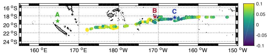
Fig. 2. Difference between in situ surface chlorophyll concentration from the underway survey and satellite-derived sea surface chlorophyll concentration from CLS ( \text{mg mEL}^{-3} )
