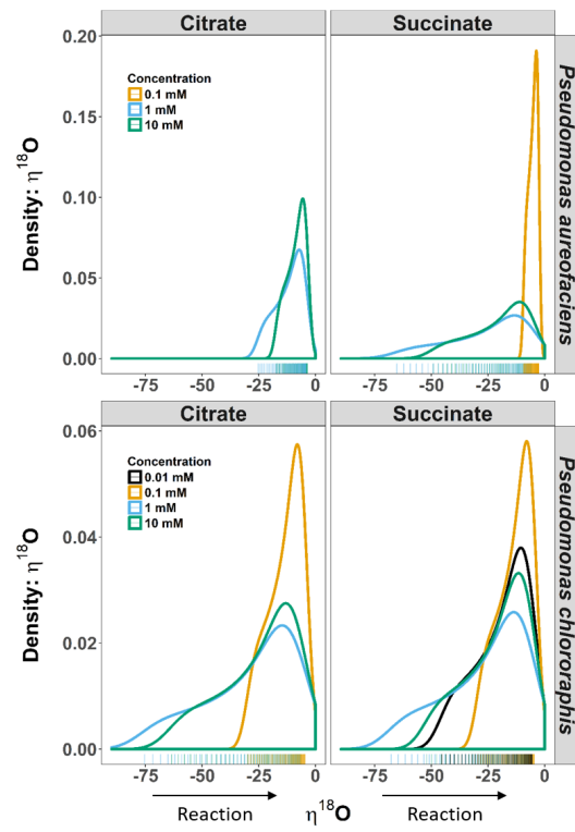
Fig. 2. Density distributions (DD) of \delta^{18}\text{O} net isotope effects ( \eta )
