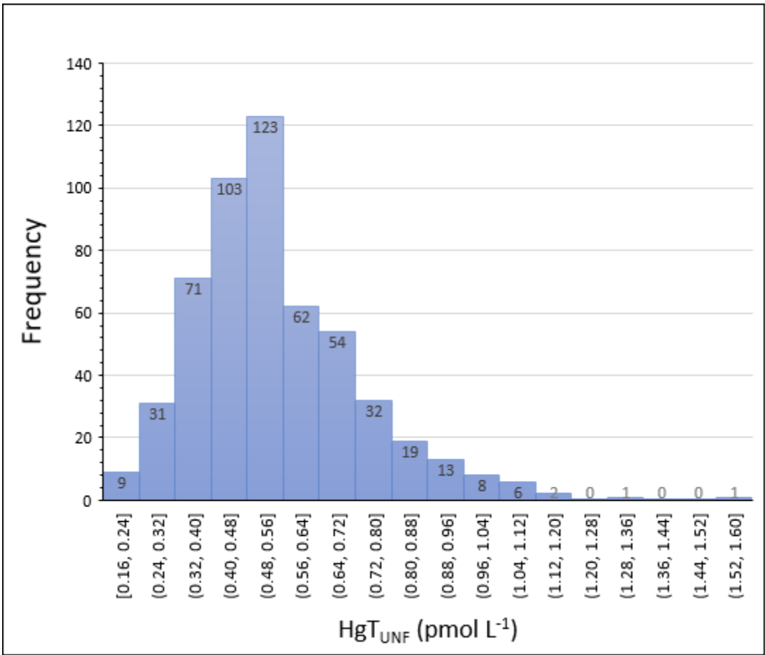
14 Figure S2. Frequency distribution of \text{HgT}_{\text{UNF}} concentrations measured in the 535 samples collected 15 along the GEOTRACES-GA01 transect.
