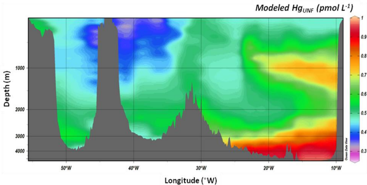
18 Figure S3. Distribution of \text{HgT}_{\text{UNF}} along the GEOTRACES-GA01 transect modelled by mixing of 19 SWTs.
