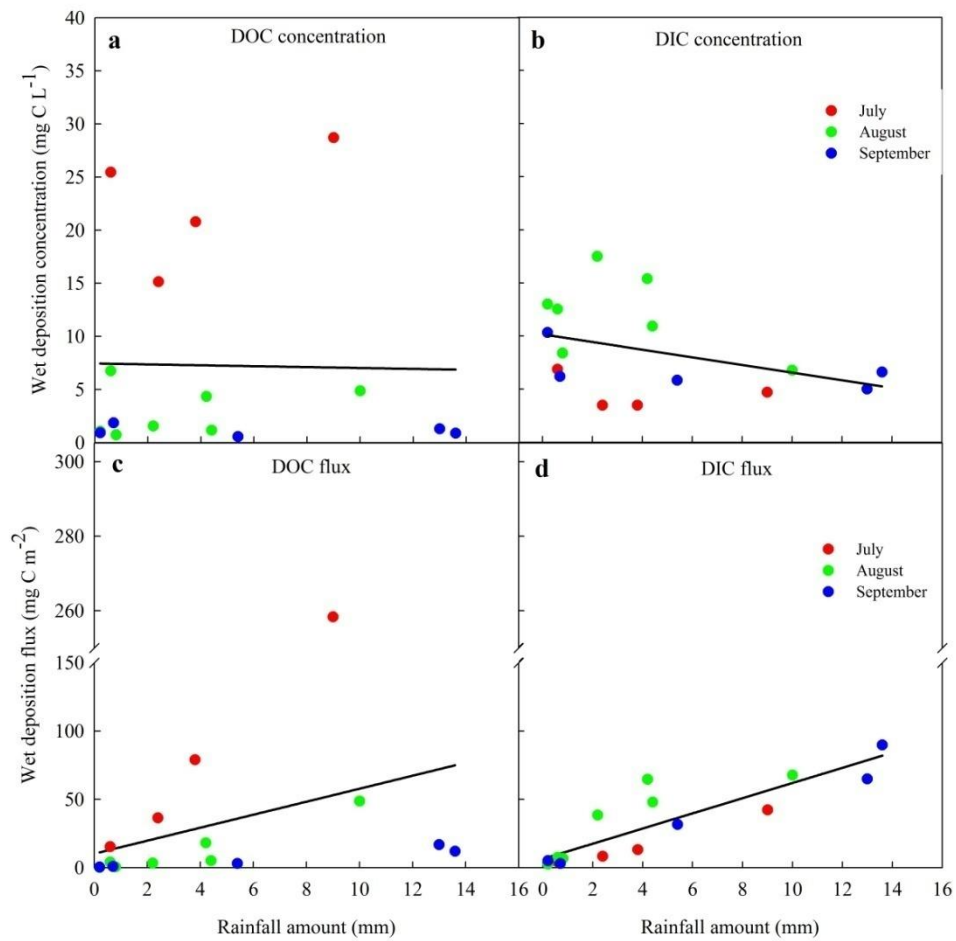
410 Figure 3 Relationships between measured parameters and rainfall amounts in a single rainfall event during July to September: (a) DOC concentration, (b) DIC concentration, (c) DOC flux and (d) DIC flux.
