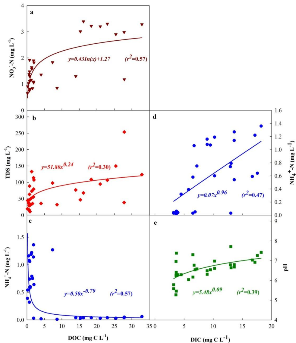
Figure 4 Significant correlations between DOC concentrations and various rainwater variables: (a) NO 3 - -N, (b) TDS, and (c) NH 4 + -N in the rainfall event samples collected during July-September. In addition, correlations between DIC concentrations with the variables: (d) NH 4 + -N and (e) pH, are also demonstrated accordingly.
