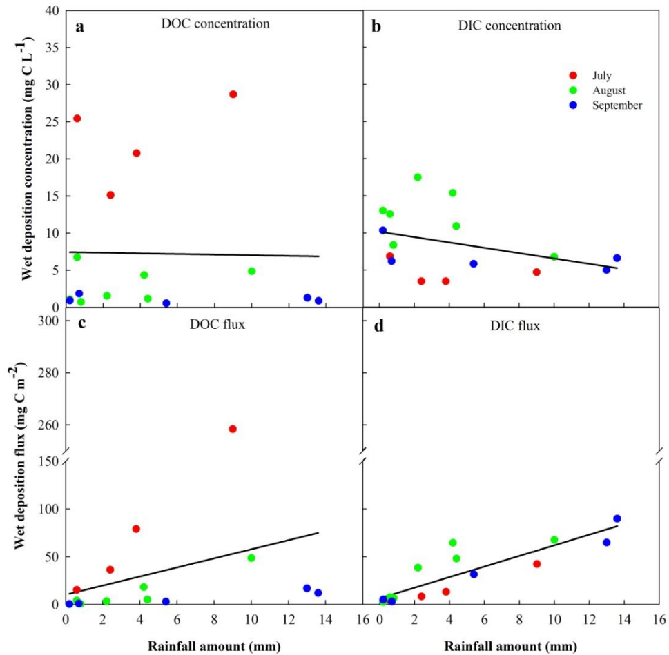
410 Figure 3 Relationships between measured parameters and rainfall amounts in a single rainfall event during July to September: (a)DOC concentration, (b)DIC concentration, (c)DOC flux and (d)DIC flux.
