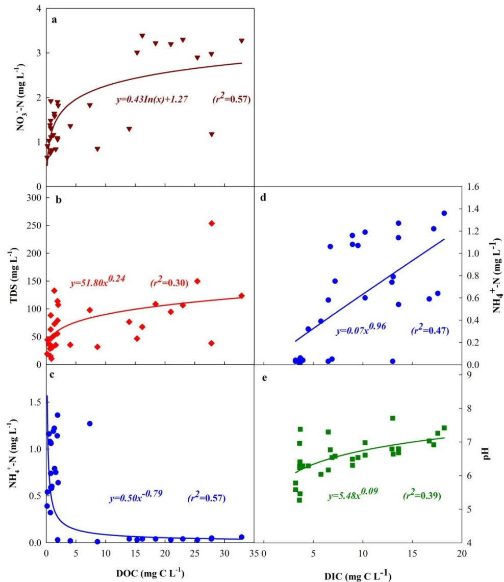
Figure 5 Significant correlations between DOC concentrations and various rainwater variables: (a) \text{NO}_3^- \text{-N} , (b)TDS, and (c) \text{NH}_4^+ \text{-N} in the rainfall event samples collected during July-September. In addition, correlations between DIC concentrations with the variables: (d) \text{NH}_4^+ \text{-N} and (e)pH, are also demonstrated accordingly.
