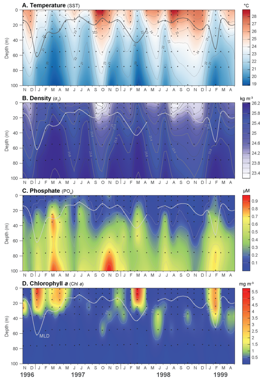
Fig. 2. Contour plots of SST (A), \sigma_T (B), \text{PO}_4 (C) and Chl a (D) over the upper 100 m from monthly water column sampling at the CARIACO station. The grey (in A) or white (B–D) line indicates the mixed layer depth (MLD).
