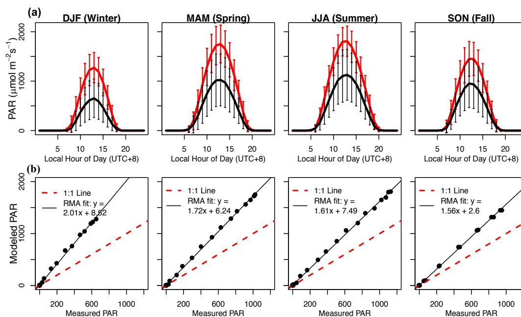
Figure 4. Derivation of PAR seasonal scaling factors. (a) Aggregated mean modeled and measured PAR for each eddy flux calibration site by season; error bars are 1-\sigma . (b) Scaling factors for each season, based on fitting modeled to measured PAR using Ranged Major Axis regression.
