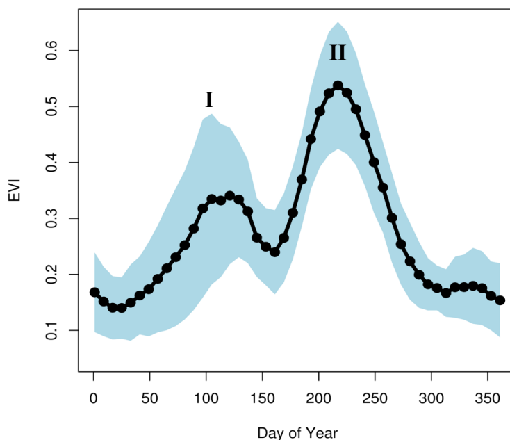
Figure 2. Average EVI in IGBP cropland class from 32N to 38N. Bimodal peak represents (I) winter wheat spring emergence and (II) corn summer emergence. Shaded blue region represents 1-\sigma of spatial and temporal average.
