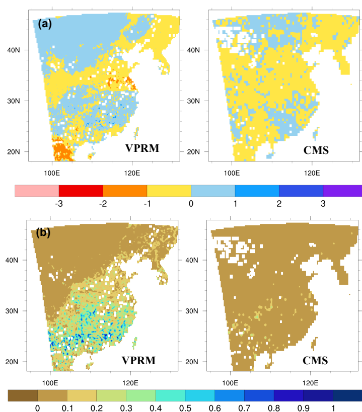
Figure 7. Annual NEE (kg C m -2 ) modeled by VPRM-CHINA and CMS reported as multi-year (2005-2009) (a) means, and (b) 1- \sigma standard deviation
