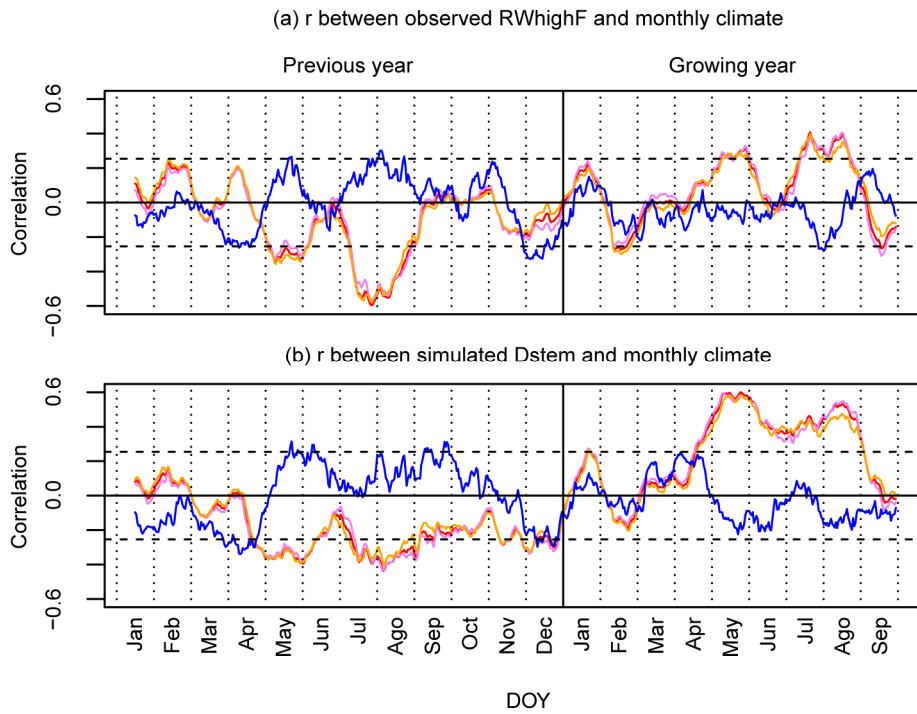
5 Figure 4: Correlation between monthly climate variables of the study area (precipitation in blue and mean, maximum and minimum temperature in red, violet and orange respectively) and the mean of the detrended series of black spruce ring growth (R highF ; a) or the simulated detrended annual carbon allocation to the stem (D stem ; b). For the climate variables, time windows of 31 days are used to obtain time series of monthly data (over the 1950-2010 period) for each day (central day), averaging the values of each window and each year. These climate time series are then detrended. Thresholds of significance ( p < 0.05 ) are shown by horizontal dashed lines.
