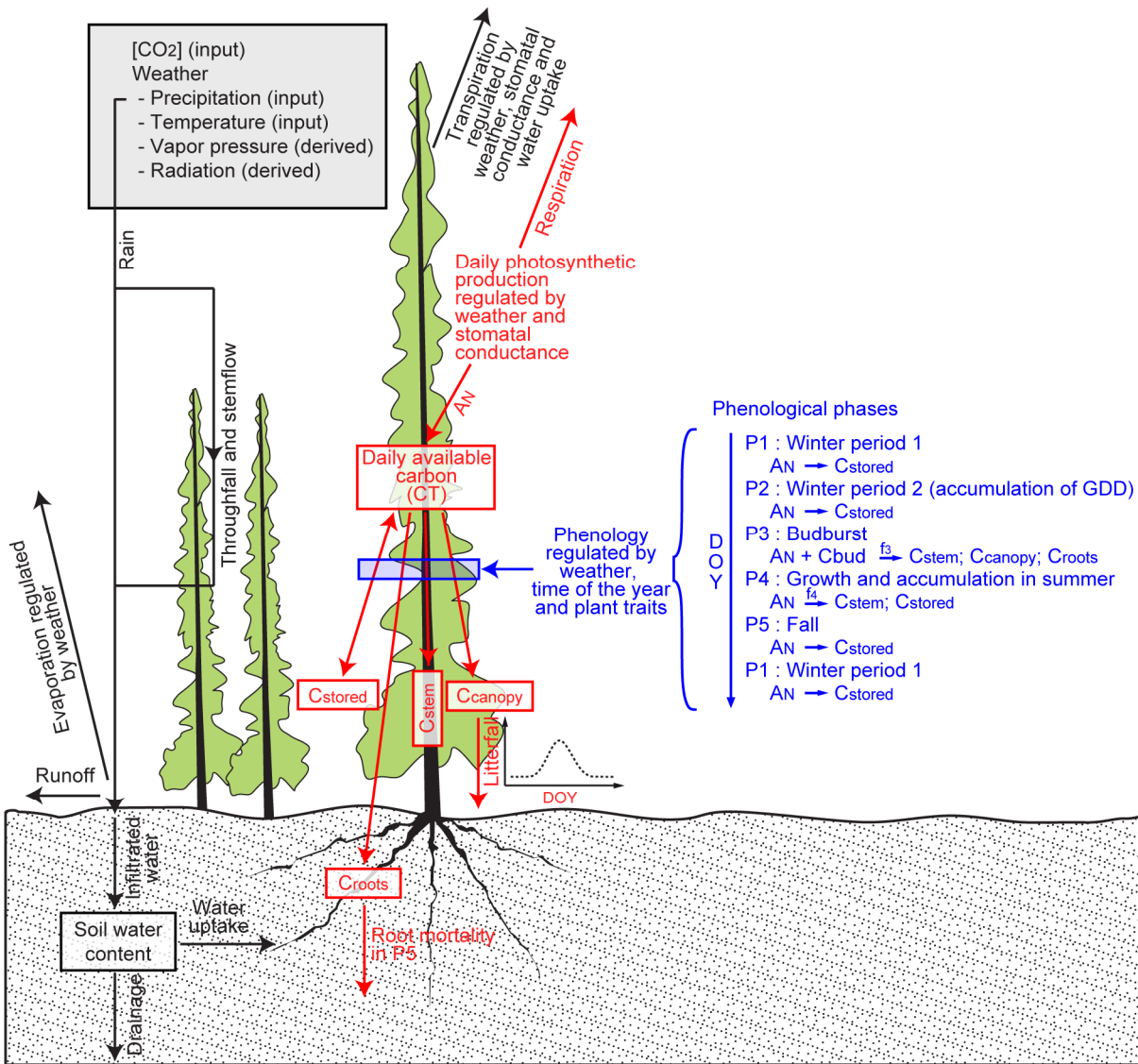
Figure 1: MAIDEN-simulated phenology (blue), water (black) and carbon (red) fluxes. AN: net photosynthesis corresponding to net primary production. Cstored, Cstem, Ccanopy, and Croots: carbon allocated daily to stored non-structural carbohydrates, stem, canopy and roots, respectively. DOY: day of the year (1-365). GDD: growing degree days. f_3 and f_4 : functions determining carbon allocation in phases 3 and 4. Cbud: amount of storage carbon that is used each day by the plant in phase 3.
