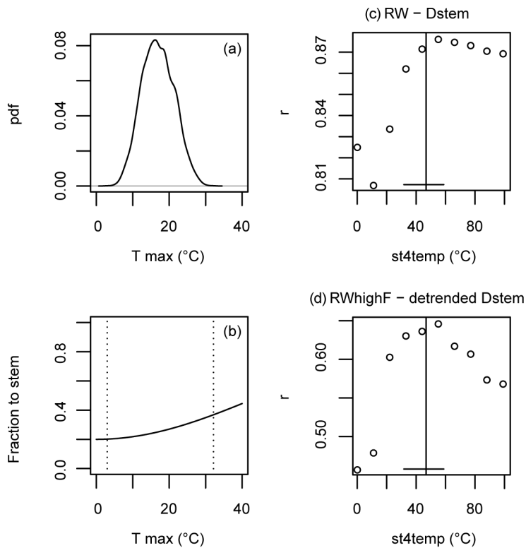
5 Figure 8: Temperature dependence of the daily partition of carbon in phase 4 (growth and accumulation phase in summer) when MAIDEN is run with the parameters of Plausible Block Stem at the center of the region with ring width data in the northern Quebec taiga. (a) Probability density of daily maximum temperature values in summer. (b) Relationship between maximum temperature values and portion of carbon allocated to the stem (Eq. (6)). The vertical dashed lines show the range of maximum temperature values. Plots c-d show how the parameter st4temp influencing this process impacts the correlations between simulated Dstem and observed ring width data (RW or RWhighF) when all other parameters are fixed to the values of Plausible Block Stem and st4temp varies over its prior acceptable range. The vertical line is the selected value for Plausible Block Stem, and the horizontal line is the 90% confidence interval based on the parameter's posterior density (Fig. S5).
