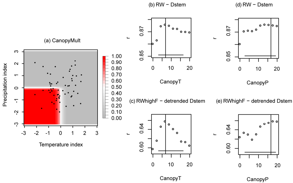
5 Figure 7: Temperature and precipitation dependence of CanopyMult (plot a; unitless multiplier; Eq. (4); CanopyT and CanopyP are those of Plausible Block Stem), which determines the yearly canopy potential amount of carbon. Previous-year mean July-August temperature indexes are on the x-axis, and previous-year April precipitation indexes are on the y-axis. Black dots are observed values in the central point of the region with ring width data. Plots b-e show how CanopyT and CanopyP (varying over their prior acceptable ranges) impact the correlations between simulated Dstem ( \text{g C m}^{-2} \text{ year}^{-1} ) and observed ring width data (RW or RWHighF; unitless indexes), when all other parameters are fixed to the values of Plausible Block Stem. The vertical lines are the selected values for Plausible Block Stem, and the horizontal lines are the 90% confidence intervals based on the parameters' posterior densities (Fig. S5).
