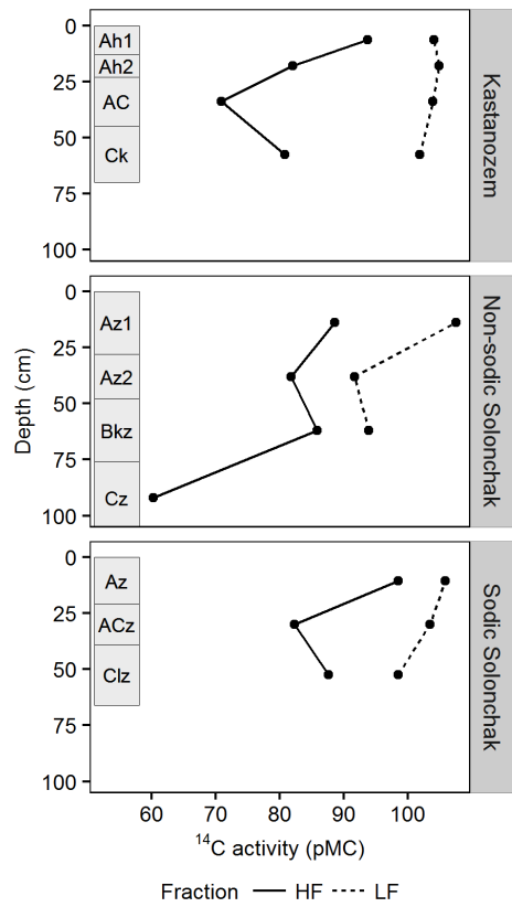
Figure 4: 14 C activity (pMC) for three soil types and two OM fractions as function of soil depth. Rectangles on the left of each panel indicate diagnostic horizons. Due to low quantity of LF material in the subsoil, 14 C activities were only analyzed until the topmost C horizon. Abbreviations: LF = light fraction, HF = heavy fraction.
