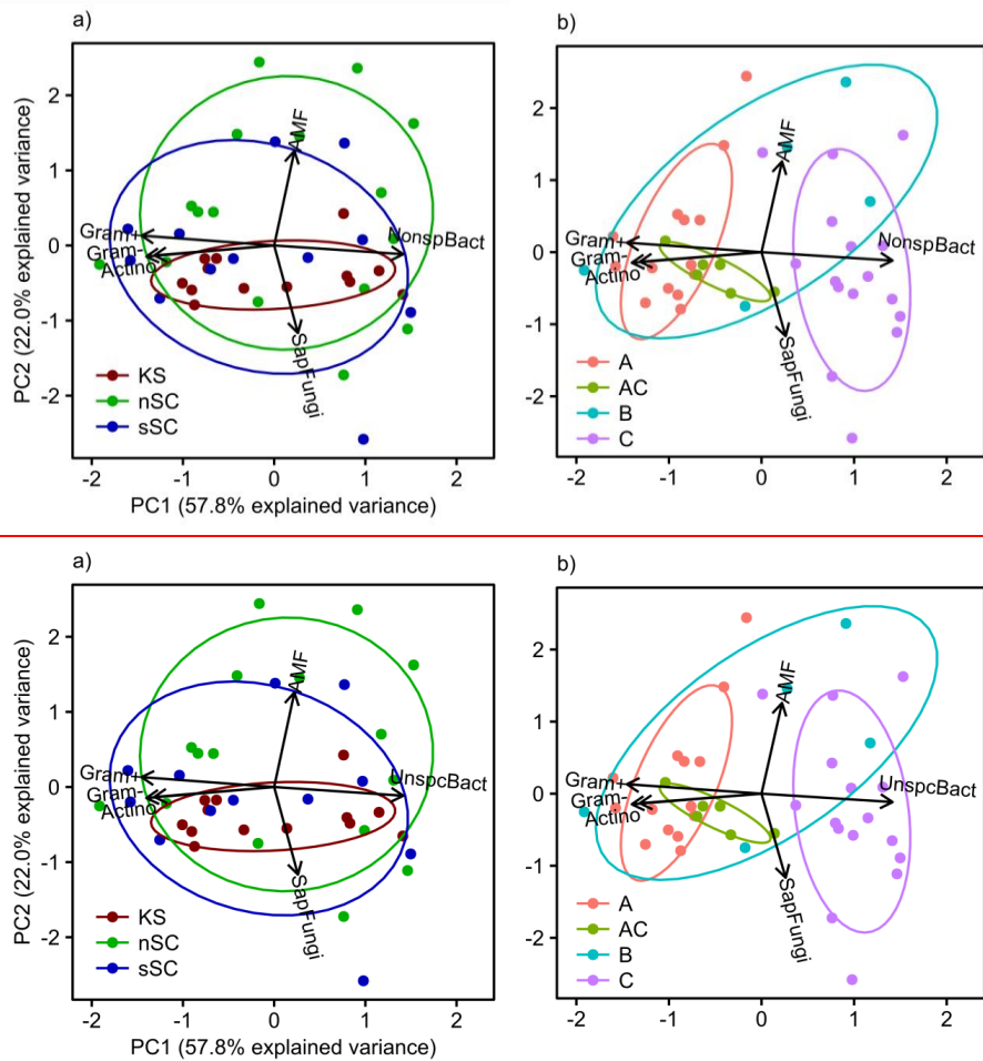
5 | Figure 6: Biplots derived from a principal components analysis of functional microbial groups as identified from PLFA analysis. Colors and 68% confidence regions are grouped by a) soil type and b) horizon. Abbreviations: KS = Kastanozem, nSC = Non-sodic Solonchak, sSC = Sodic Solonchak, Gram+ = gram-positive bacteria, Gram- = gram-negative bacteria, Actino = actinomycetes, SapFungi = saprotrophic fungi, NonUnspeBact = nonspecific unspecific bacteria, AMF = arbuscular mycorrhizal fungi.
