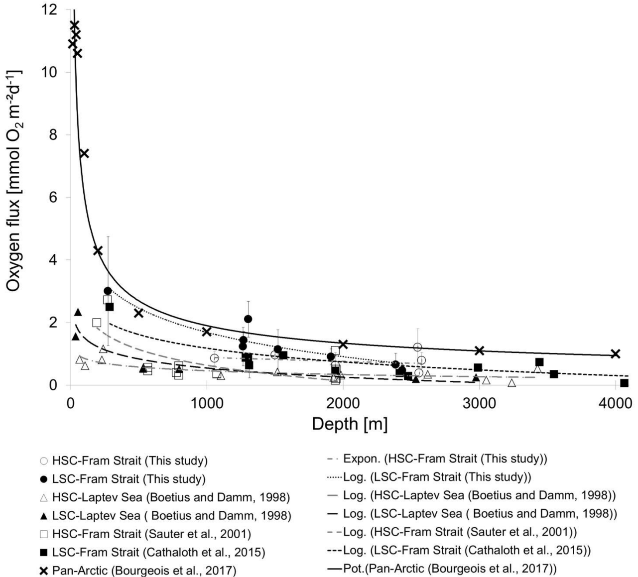
Figure 6. Sediment oxygen uptakes in different water depths (15 – 4000 m) in areas with a high sea-ice concentration (HSC, >30 % sea-ice concentration) and a low sea-ice concentration (LSC, <30 % sea-ice concentration) from this study and from literature data for the Laptev Sea, Fram Strait, and Pan-Arctic region and related regressions for HSC and LSC sea-ice categories from this study and from literature data for the Laptev Sea, Fram Strait, and Pan-Arctic region and related regressions. HSC regression from this study: y = -0.124 \ln(x) + 1.7388 ( R^2 = 0.0255 ); LSC regression from this study: y = -1.119 \ln(x) + 9.4144 ( R^2 = 0.8695 ); HSC regression from Sauter et al. (2001): y = -0.727 \ln(x) + 5.6587 ( R^2 = 0.5026 ); LSC regression from Cathalot et al. (2015): y = -0.63 \ln(x) + 5.534 ( R^2 = 0.7013 ); HSC regression from Boetius and Damm (1998): y = -0.172 \ln(x) + 1.6496 ( R^2 = 0.6074 ); LSC regression from Boetius and Damm (1998): y = -0.421 \ln(x) + 3.4515 ( R^2 = 0.8428 ); Pan-Arctic regression from Bourgeois et al (2017): y = 7.1338e^{-6E-04x} ( R^2 = 0.7288 ). Regression types were chosen based on best fit ( R^2 ). The model of Bourgeois et al. (2017) included DOU and TOU values, while all other references refer only to DOU values.
