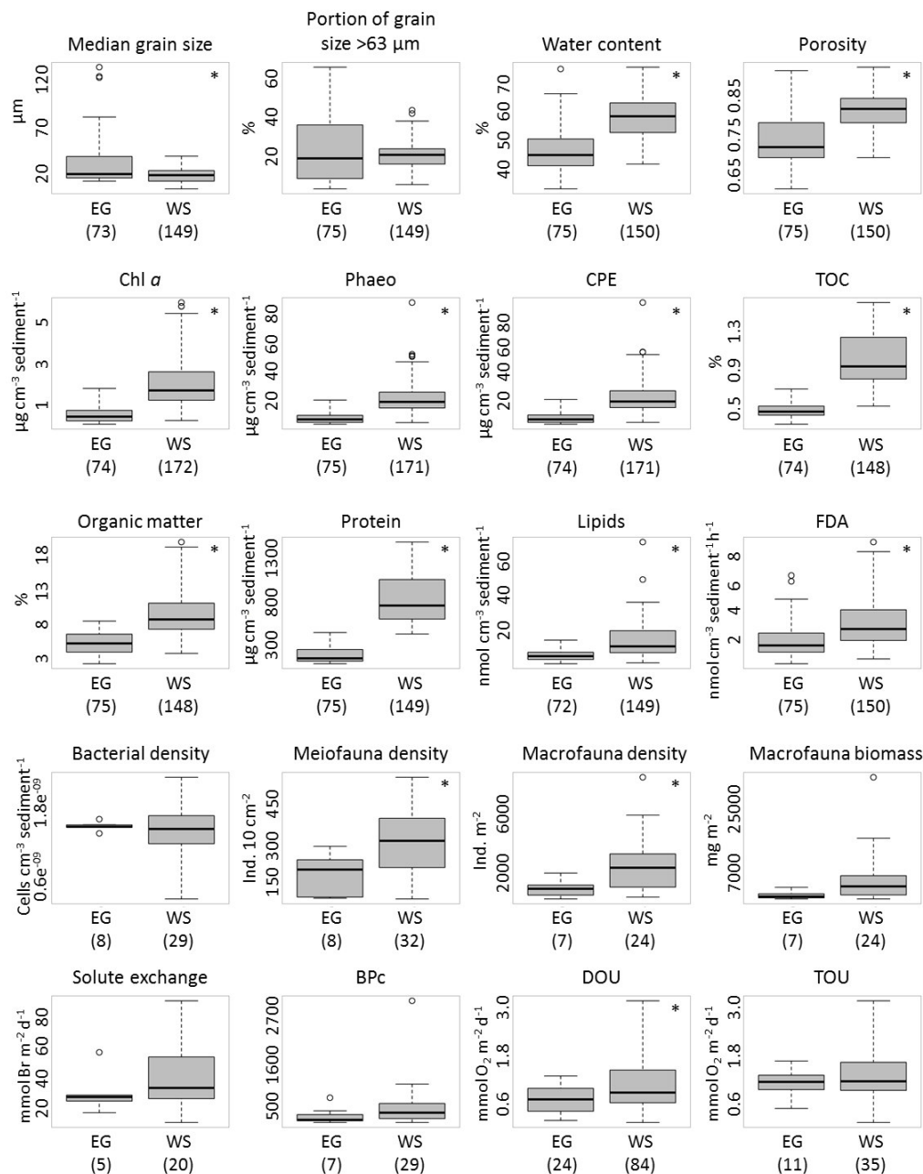
Figure 3. Boxplots of sediment properties, biogenic compound values (Chl a = chlorophyll a , Phaeo = phaeophytin, CPE = chloroplatic pigment equivalents, TOC = total organic carbon, FDA = bacterial enzymatic turnover rates calculated using the fluorogenic substrate fluorescein-di-acetate), benthic community data and function (BPC = bioturbation potential), and oxygen fluxes (DOU = diffusive oxygen flux, TOU = total oxygen flux), of the East Greenland (EG) and West Spitsbergen (WS) area. For a detailed description of which stations were included at which site, see section 2.1. The number of observations is given in brackets below the area. Parameters showing significant differences between areas are marked with an asterisk. For comparability, the WS site does not contain values from SV I station.
