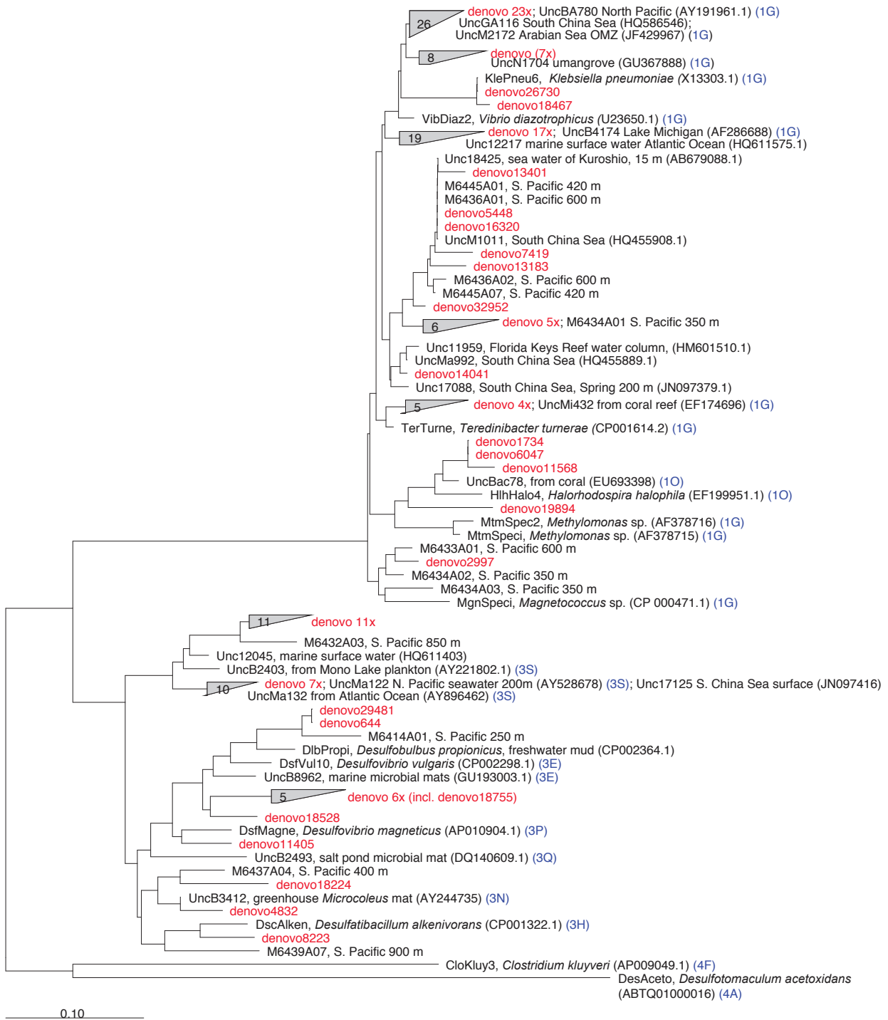
Figure 4: A nifH amino acid neighbor-joining tree with 100 most abundant OTUs from this study shown. Sequences 'denovo-' shown in red are randomly chosen representative sequences from these OTUs (OTUs binned at 97% identity). The clusters in the tree are grouped at an approximately >95% sequence identity. The tree includes reference sequences (if uncultivated, names of these sequences start with 'Unc'). The reference sequences are shown with accession numbers from the nifH database and with the cluster identifier shown in blue if indicated in the nifH database. Additional sequences are included from a previous study in the South Pacific mesopelagic layers (Benavides et al. 2015); these clones are labeled with the original clone names M64XXAXX and depths.
