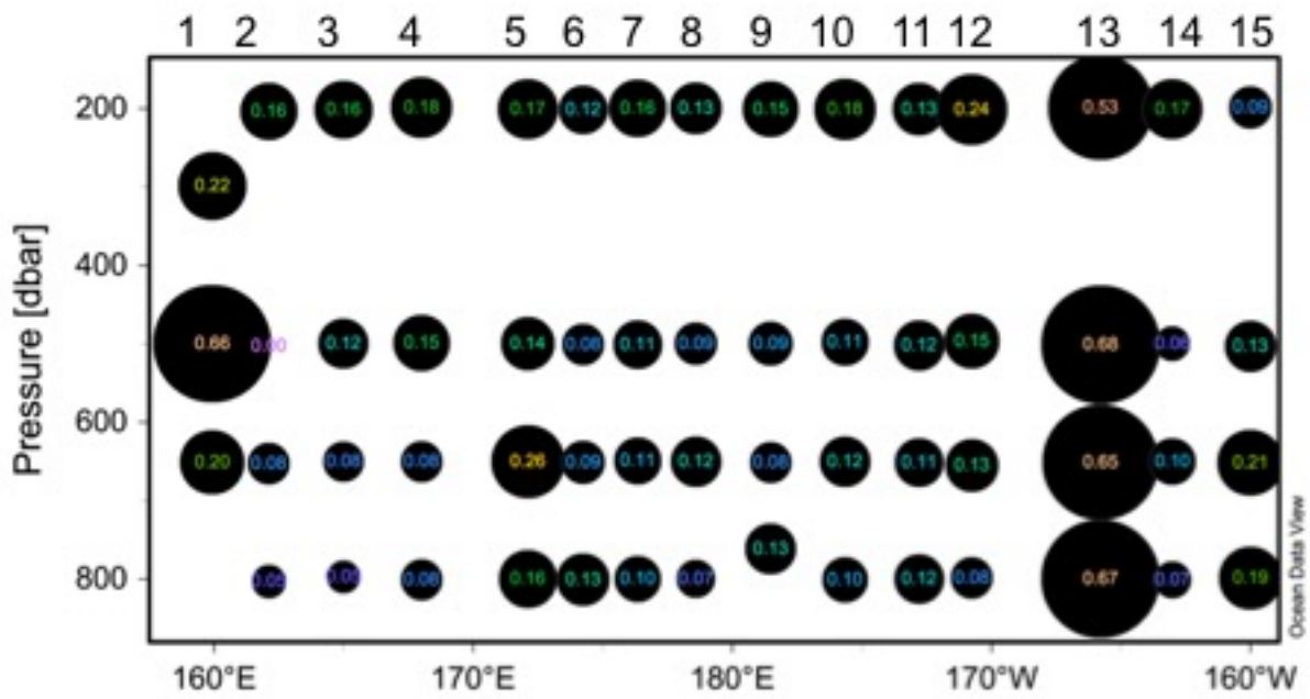
Figure 1: Longitudinal section of N 2 fixation (nmol N L -1 d -1 , rates displayed as numbers overlying sized circles. For reference, the station numbers are displayed on top of the panel.
