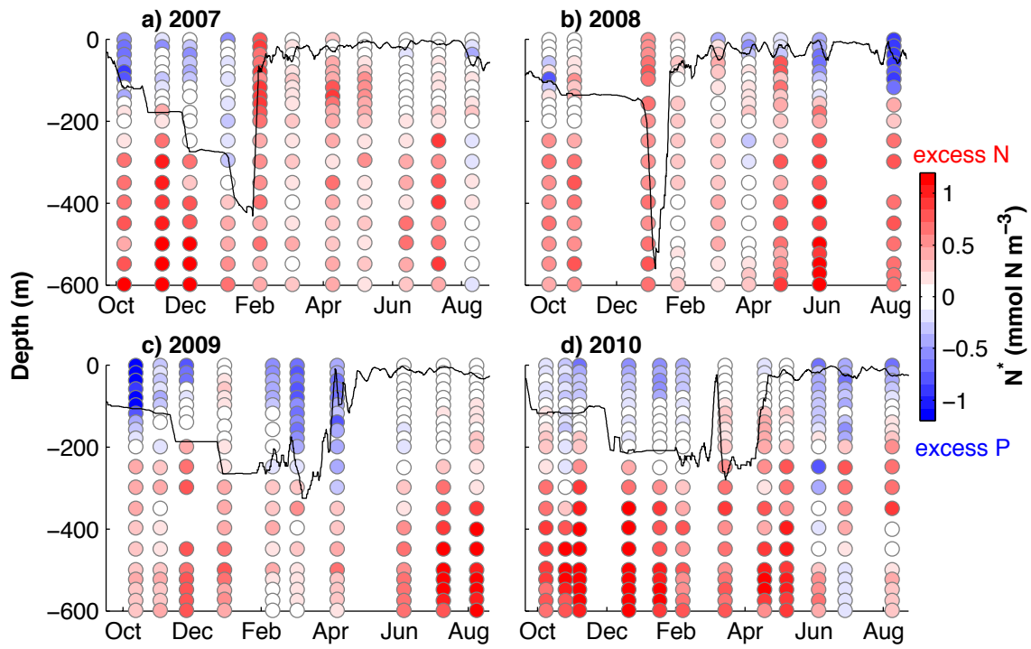
Figure 3: N^* calculated from \text{NO}_3 and \text{PO}_4 profiles from Figure 2. The black lines show estimated mixed layer depths using a maximum density gradient criterion.
