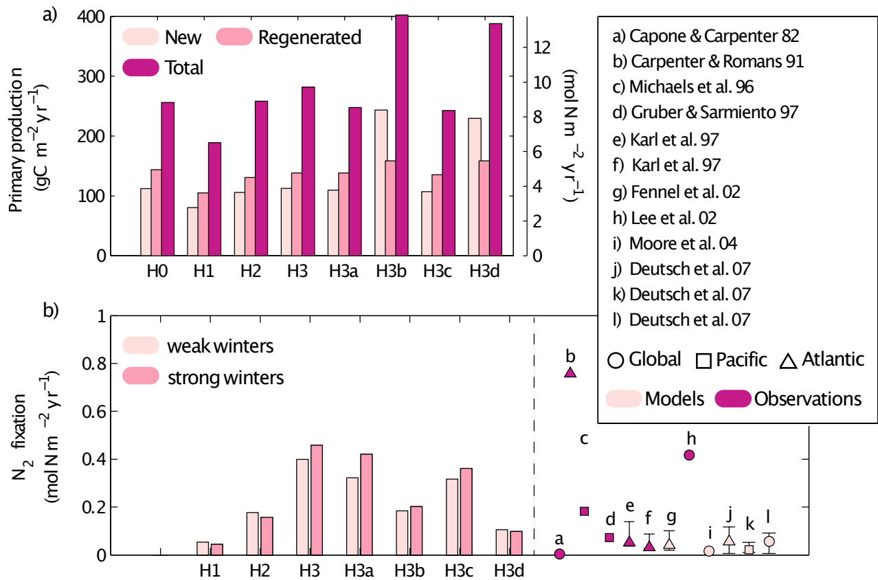
Figure 11: Simulated new, regenerated, and total primary production (a) and N 2 fixation rates (b) obtained by the different simulations (see Table 1 for key to different simulations). A summary of previous estimates of N 2 fixation rates in observational and model studies is included in (b). Redfield C:N ratio is used to transform the model results nitrogen units to carbon units. Control versions H0' and H3' are not shown.
