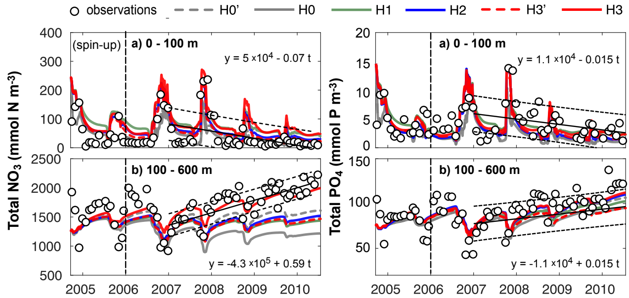
Figure 5: Observed and simulated vertically integrated \text{NO}_3 and \text{PO}_4 between 0 – 100 m and between 100 – 600 m using model versions H0 (no nitrogen fixers), H0' (no sediment denitrification – no fixers), H1 (generic autotrophic fixer), H2 (unicellular and colonial autotrophic fixers), H3' (non- \text{N}_2 -fixing heterotrophic, and unicellular and colonial autotrophic fixers), H3 (heterotrophic, and unicellular and colonial autotrophic fixers). Tick marks are placed on the April 1 st of every year.
