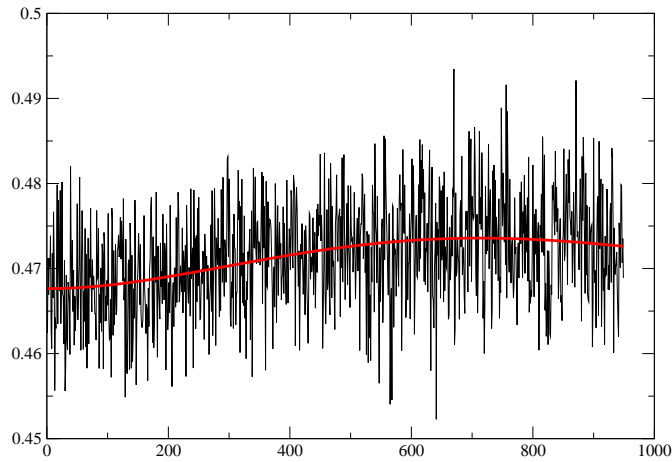
Fig. 1. Efficiency of the biological pump based on eq. 4.1.1 in Sarmiento and Gruber (2006) and global mean NO 3 from 0-100m (surface) and 100-200 m (deep) as in Fig. 4.1.7 in Sarmiento and Gruber (2006). X-axis in years/10, 950 = 0 kyr BP.
