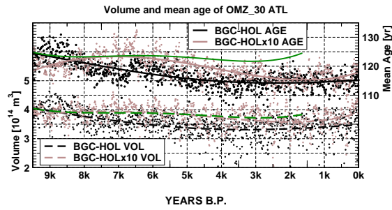
Fig. 14. As Fig. 12 but for the Atlantic in the area of 5°W - 15°E, 30°S - 5°N, 0 - 1000 m depth. OMZ-volume for a threshold of 30 \mu\text{mol l}^{-1} in 10^{14} \text{ m}^3 and water mass age in years.
