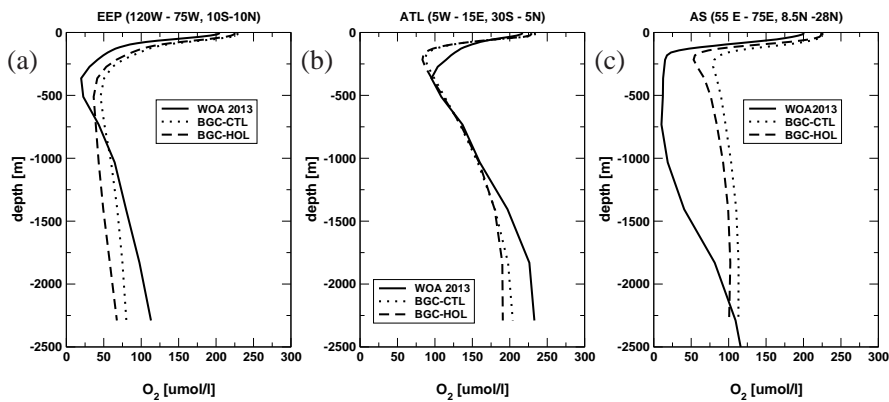
Fig. A.1. Simulated and observation-based profiles of average O 2 -concentration in \mu\text{mol l}^{-1} in the three major oxygen minimum zones in the world ocean for (a) the eastern equatorial Pacific, (b) the tropical South Atlantic, and (c) the Arabian Sea. Based on observations (WOA2013, Garcia et al., 2013, solid), and from experiments BGC-CTL (dotted) and BGC-HOL (dashed) averaged over the last 200 years.
