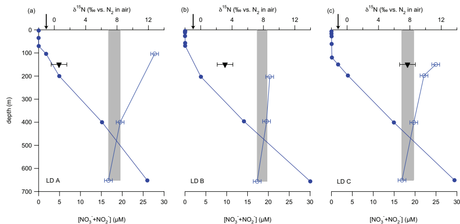
Figure 1. \text{NO}_3^- + \text{NO}_2^- concentration (filled circles), \text{NO}_3^- + \text{NO}_2^- \delta^{15}\text{N} (open circles), and \text{PN}_{\text{sink}} \delta^{15}\text{N} (filled inverted triangles) from OUTPACE “long duration” (LD) stations A (a), B (b), and C (c). Error bars represent 1 standard deviation, and are smaller than symbol size for \text{NO}_3^- + \text{NO}_2^- concentration. The range of \text{NO}_3^- + \text{NO}_2^- \delta^{15}\text{N} end-member values used for \delta^{15}\text{N} budget calculations are represented by shaded regions. The \text{N}_2 fixation end-member \delta^{15}\text{N} value, -1\text{‰} , is represented by the arrow on the upper x-axis.
