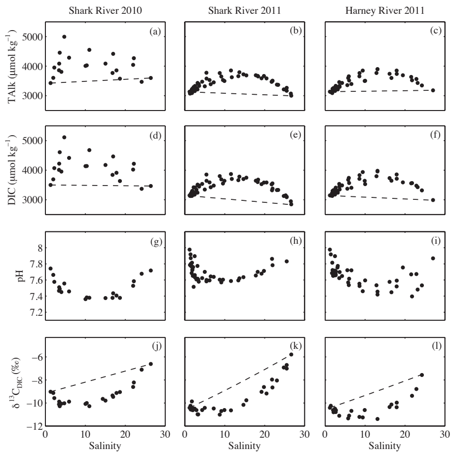
790 Figure 3. Distribution of TALK (a-c), DIC (d-f), pH (g-i) and \delta^{13}\text{C}_{\text{DIC}} (j-l) along the salinity gradient in the Shark and Harney Rivers during the 2010 (SharkTREx 1) and 2011 (SharkTREx 2) campaigns. During SharkTREx 1, TALK and pH were measured at FIU, and DIC was calculated using CO2SYS (Pierrot et al., 2006). During SharkTREx 2, DIC and TALK were measured at NOAA/AOML, and pH was calculated using CO2SYS. The dashed lines indicate the distribution expected for conservative mixing.
