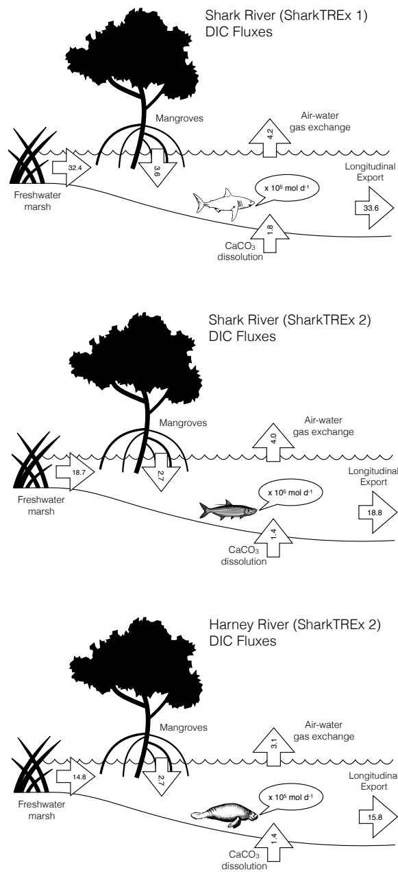
795 Figure 5. Diagrams showing the main DIC fluxes (in 10^5 \text{ mol d}^{-1} ) entering and exiting the Shark and Harney Rivers during SharkTREx 1 and 2. Fluxes from the freshwater marsh were assumed to be fluxes estimated from the conservative DIC curves.
