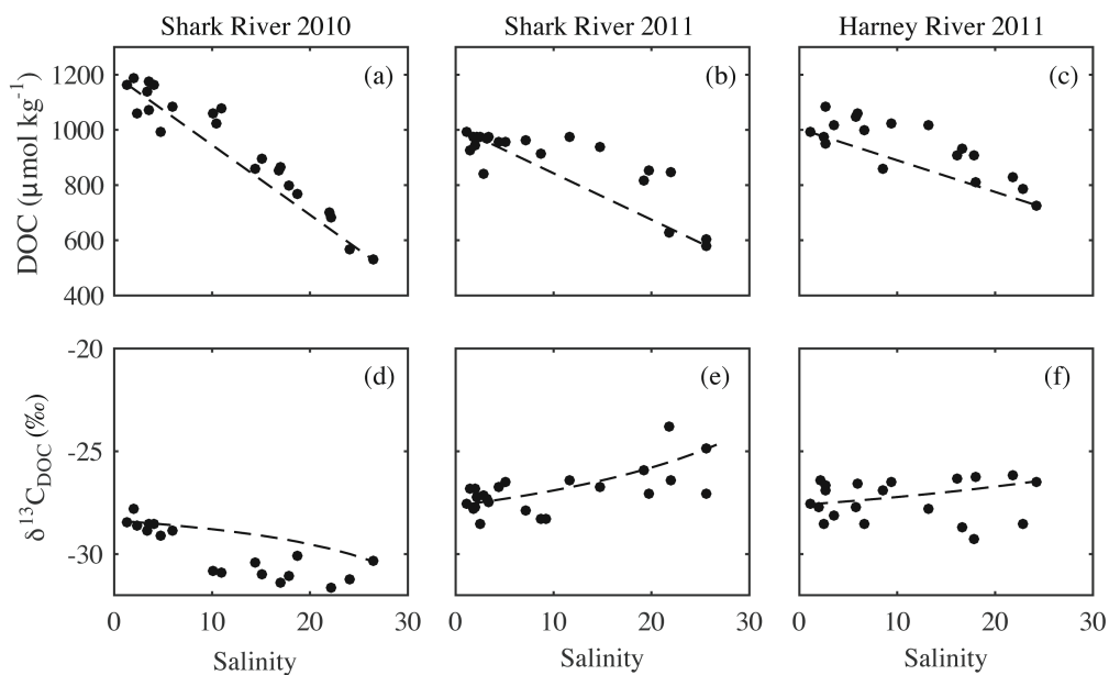
Figure 4. Distribution of DOC and \delta^{13}\text{C}_{\text{DOC}} along the salinity gradient in the Shark and Harney Rivers in samples
