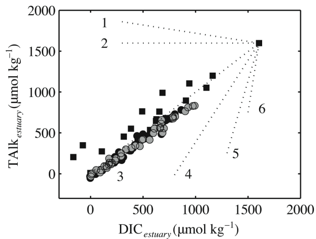
Figure 6. (a) Covariation of \text{DIC}_{\text{estuary}} and \text{TAlk}_{\text{estuary}} . Black squares are samples from the Shark River during SharkTREx 1, 800 and black and gray circles are from the Shark and Harney Rivers, respectively, during SharkTREx 2. Dotted lines represent the theoretical covariation of DIC and TAlk for different biogeochemical processes: 1) aerobic respiration; 2) \text{CO}_2 emission, 3) sulfate reduction, 4) \text{CaCO}_3 dissolution, 5) manganese reduction, and 6) iron reduction.
