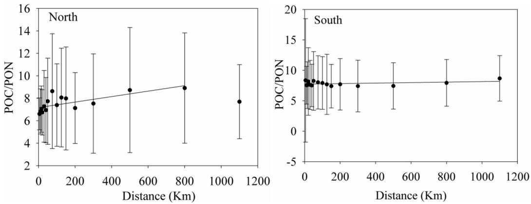
235 Figure 6 The variation of POC/PON with the distance from the shore to open sea. The relationships between POC/PON and distance are POC/PON=0.0024 \cdot D+7.1764 ( R^2=0.519 , North hemisphere) and
