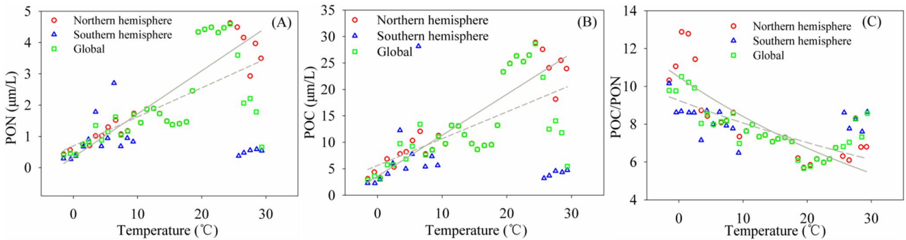
Figure 10 Relationships between POC, PON, and POC/PON and temperature (T). POC, PON and POC/PON are highly correlated to temperature in the northern hemisphere (solid line), with relationships of PON=0.142*T+0.260 ( R^2=0.74 ), POC=0.788*T+3.340 ( R^2=0.74 ) and POC/PON=11.88*T^{-0.190} ( R^2=0.81 ), respectively. There is almost no correlation in the southern hemisphere, with correlation coefficients of -0.11, -0.08 and -0.31 for PON, POC and POC/PON, respectively. The relationships between POC, PON, and POC/PON and T at a global scale (dash line) are PON=0.093*T+0.697 ( R^2=0.42 ), POC=0.507*T+5.630 ( R^2=0.41 ) and POC/PON=10.02*T^{-0.122} ( R^2=0.57 ).
