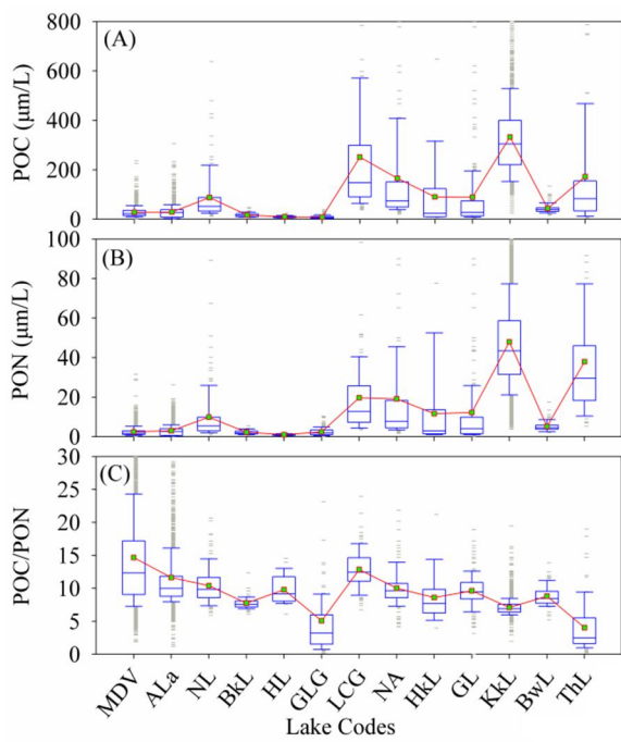
Figure 7 Variation of PON, POC and POC/PON in lake waters. The lakes are mainly located in the northern hemisphere. Eutrophic, small, large, and shallow lakes are included in the dataset. MDV is McMurdo Dry Valleys Lakes (Antarctica), ALa is Alaskan Lakes(USA), NL is Norwegian Lakes (Norway), NA is Northern American Lakes (USA), HKL is Hokkaido Lakes (Japan), LCG is Lacustrine Central Group (USA), KkL is Lake Kasumigaura (Japan),
