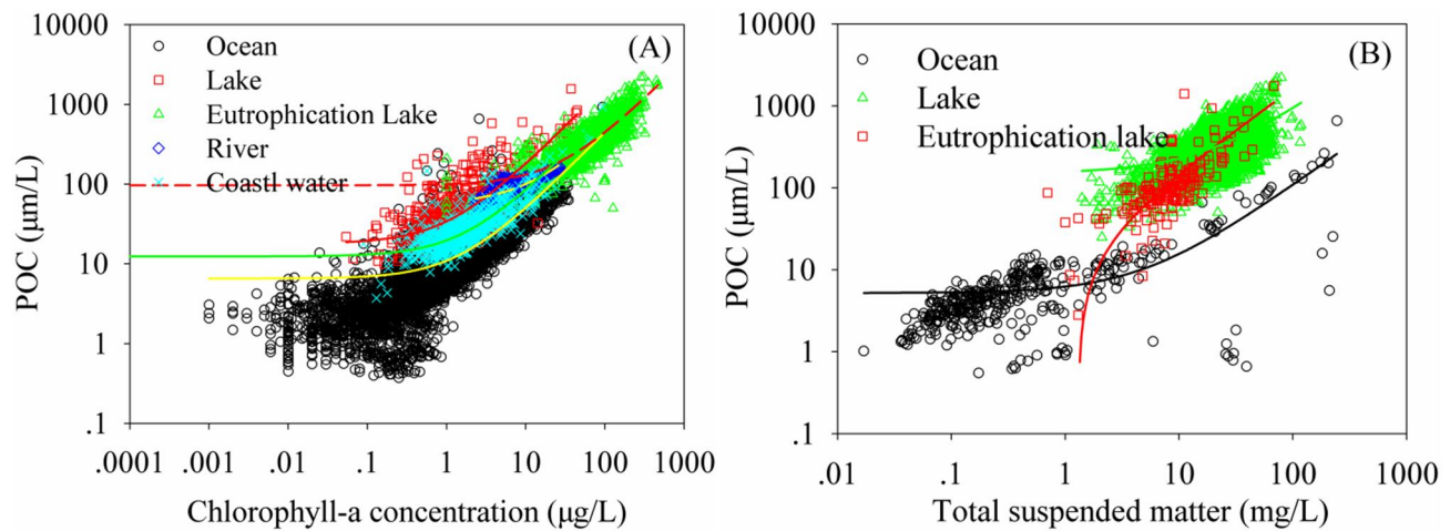
Figure 11 (A) Comparison of the relationships between POC and chlorophyll-a concentration ( C_{\text{Chl-a}} ) for oceans, lakes, eutrophic lakes, rivers and coastal waters. (B) Comparison of the relationship between POC and total suspended matter
