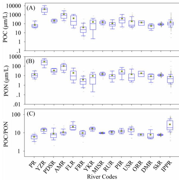
Figure 8 Variation of PON, POC and POC/PON in river waters. PR is Pearl River (China), YZR is Yanagtzte River (China), PDSR is paraiba do sul River (Brazil), AMR is Amazon River (Brazil), FLR is Fly River (Papua New Guinea), FRR is Fraser River (Canada), YKR is Yukon River (USA), MISR is Mississippi River (USA), RUR is Russian rivers (Russian), PIR is Ping River (Thailand), USR is Union and Skokomish River (USA), ORR is Orinoco river (Venezuela), DMR is Mandovi river (India), SkR is Skidaway River (USA), IPPR is Ipswich and Parker rivers (USA).
