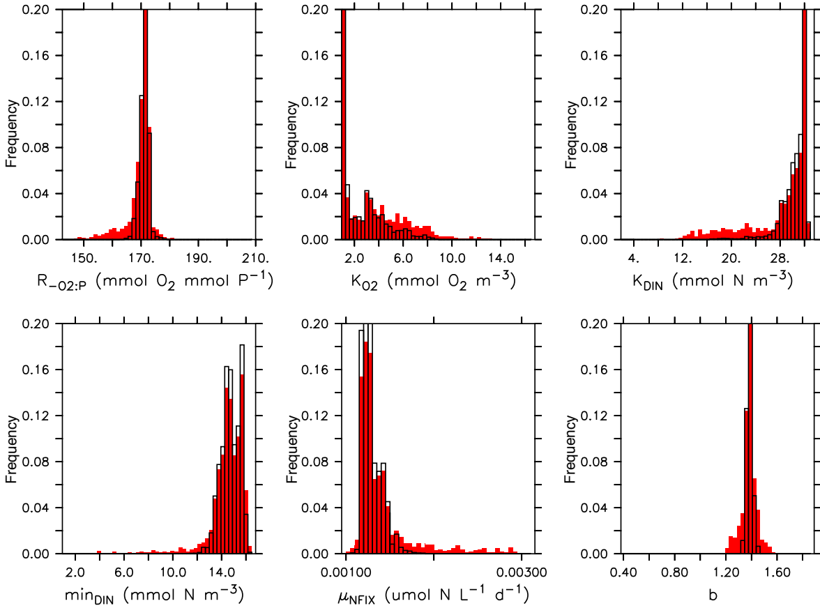
Figure 1. Parameter distribution of model simulations obtained during the optimisation of MOPS oD , whose misfit do not exceed a threshold limit of \Delta J = 1.1 J^* (10%, red bars) or \Delta J = 1.01 J^* (1%, open bars) of the minimum misfit J^* . For the projection parameters of all model simulations in the optimisation trajectory were grouped into 50 classes.
