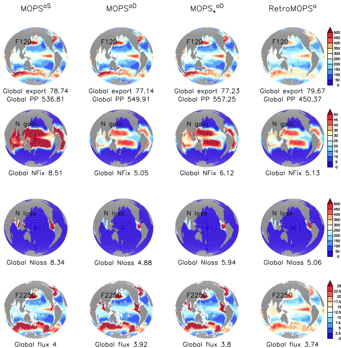
Figure 2. Biogeochemical fluxes of MOPS oS , MOPS oD , MOPS *oD and RetroMOPS o . Top: Export production (here: sedimentation at 120 m). Second row from top: nitrogen fixation. Third row from top: fixed nitrogen loss through pelagic denitrification. Bottom: sedimentation at 2250 m. All fluxes in \text{mmol N m}^{-2} \text{y}^{-1} . Each subpanel also gives the global flux in \text{Tmol N y}^{-1} .
