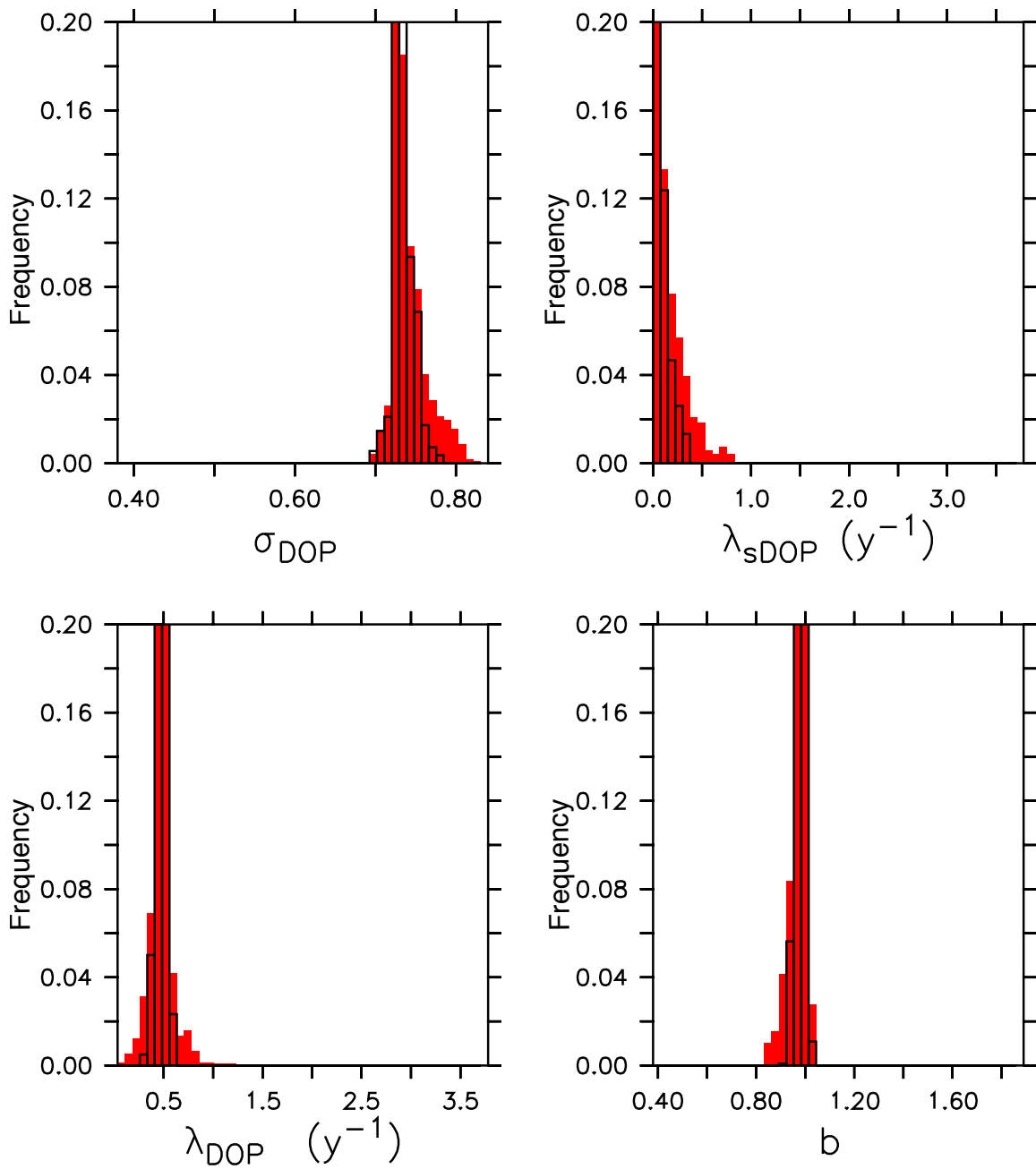
Figure 7. As Fig. 1, but for optimisation RetroMOPS°.
