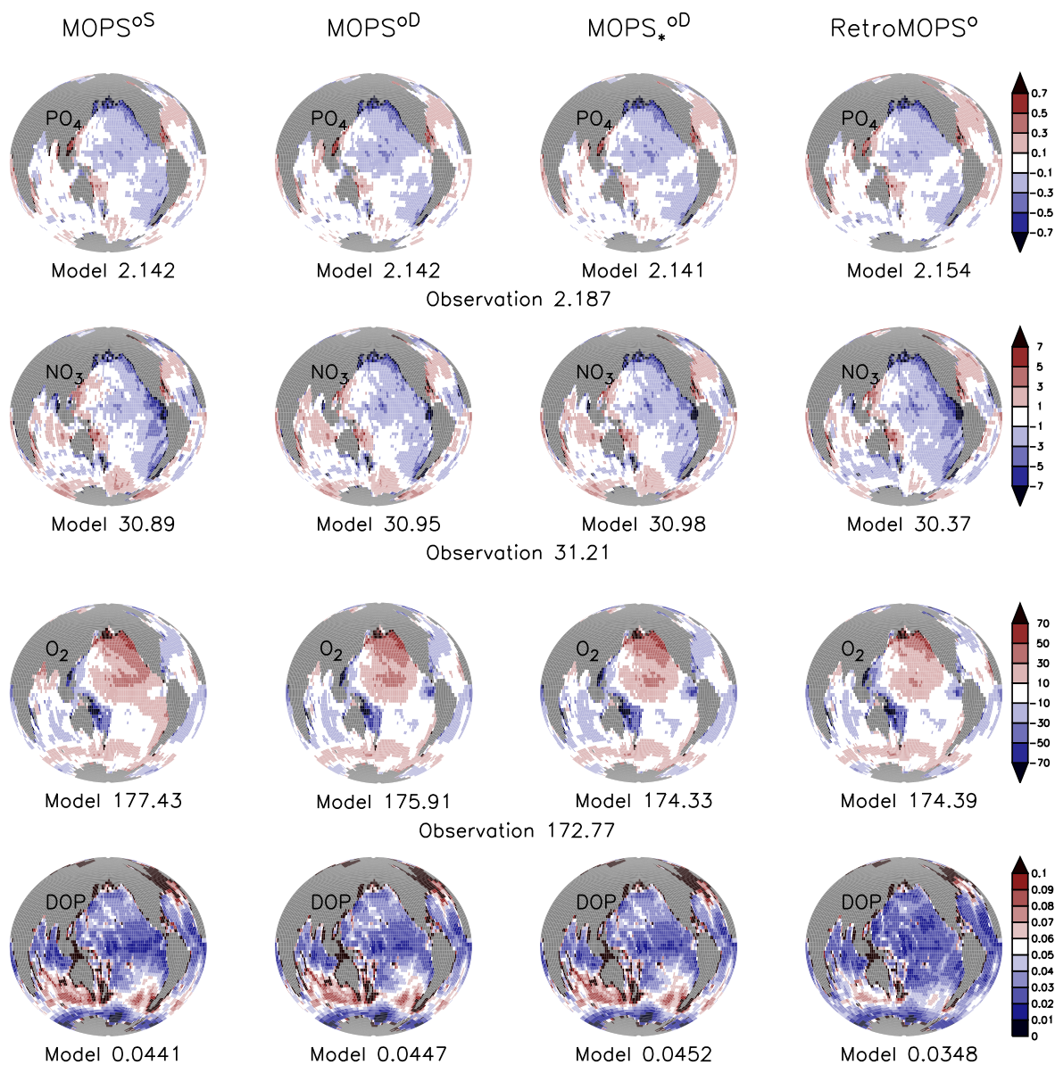
Figure 3. Vertically averaged tracers of MOPS oS , MOPS oD , MOPS *oD and RetroMOPS o . Top: phosphate. Second row from top: nitrate. Third row from top: oxygen. Bottom: DOP. Phosphate ( \text{mmol P m}^{-3} ), nitrate ( \text{mmol N m}^{-3} ) and oxygen ( \text{mmol O}_2 \text{ m}^{-3} ) are expressed as deviation from observations (Garcia et al., 2006a, b), DOP is given in absolute concentrations ( \text{mmol P m}^{-3} ). Each subpanel also gives the global average tracer concentration in \text{mmol m}^{-3} .
