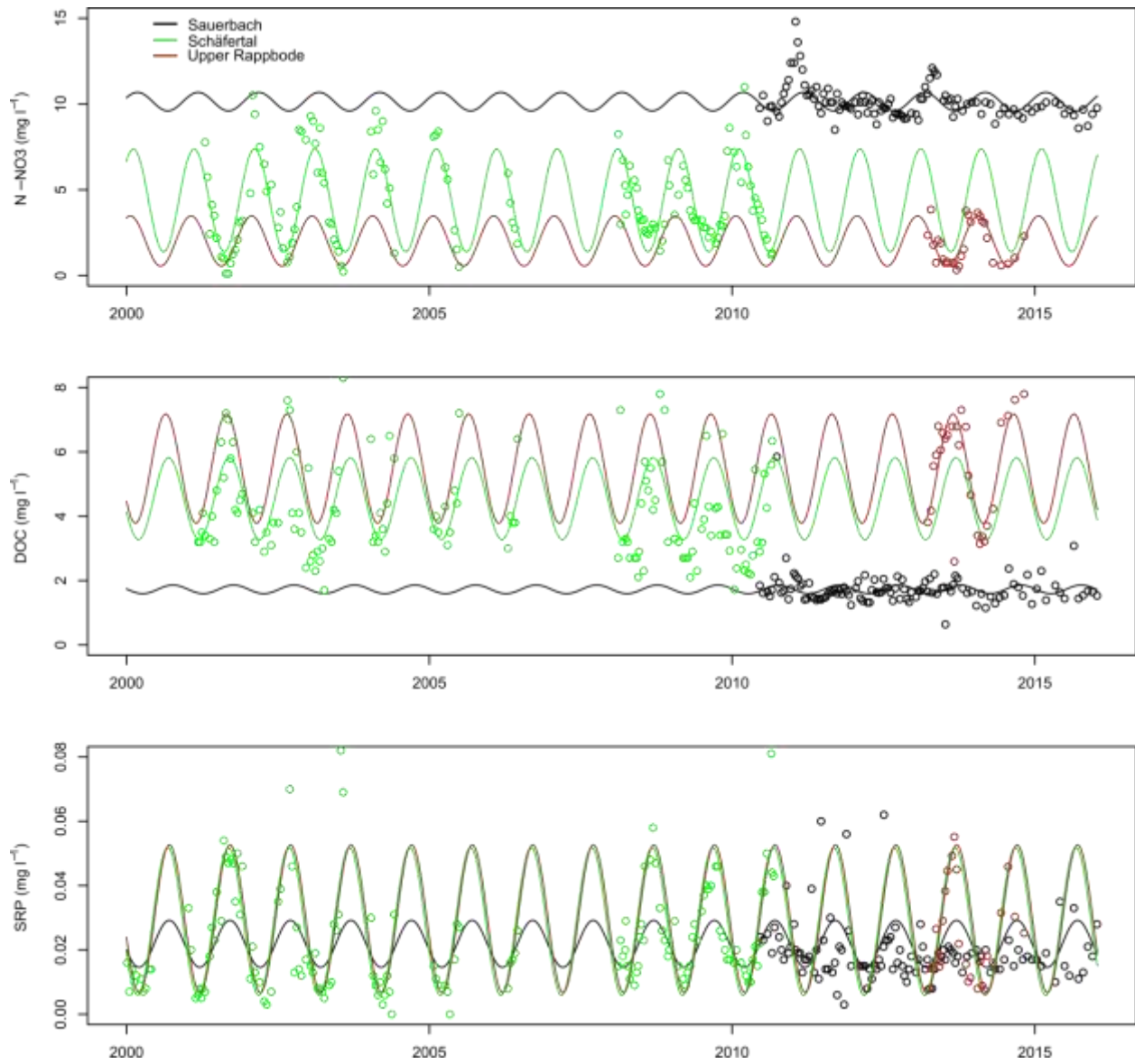
Figure S1: Grab sampling data in 3 headwater catchments and cosine fitting.
