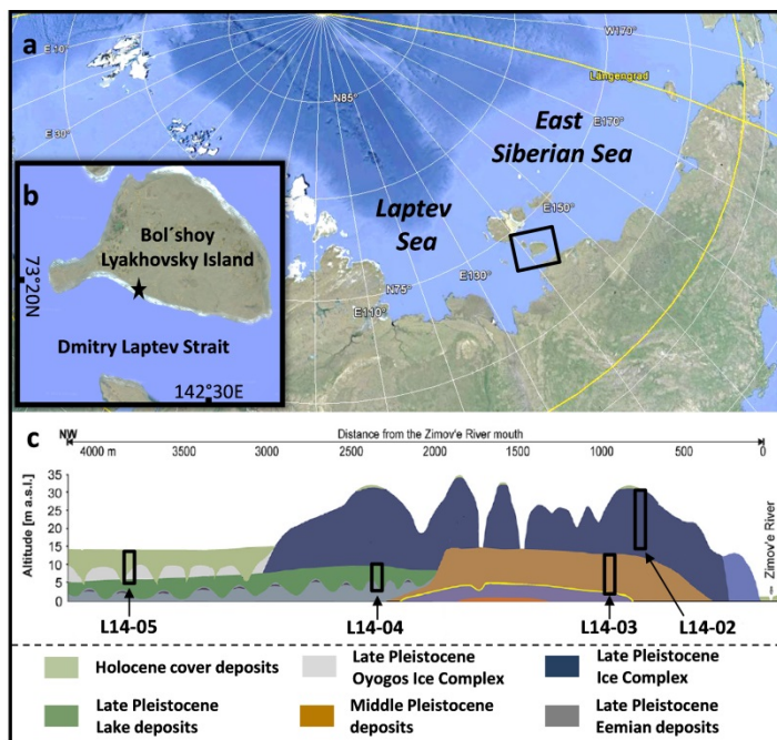
Figure 1: (a) Position of Bol'shoi Lyakhovskiy Island in the Siberian Arctic. (b) Study site on Bol'shoi Lyakhovskiy Island, indicated by a black star, (c) and location of the drilled cores comprising different age intervals (L14-05, L14-02, L14-03 and L14-04) modified after Wetterich et al. (2014) and Schwamborn and Wetterich (2015).
