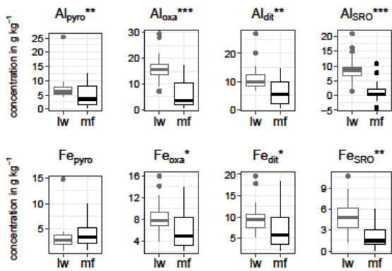
Figure 45: Distribution of Fe and Al species concentrations in the B horizon of lw and mf plots. Boxplots represent the distribution around the median values. “Pyro”, “oxa” and “dit” subscripts mention the type of extractions used for isolating Fe and Al species (respectively pyrophosphate, oxalate and dithionite-citrate). “SRO” stand for “short-range order species (Al SRO =Al oxa -Al pyro , Fe SRO =Fe oxa -Fe pyro ). Asterisks indicate significant difference using mixed models (see Material and Methods), with *: p-value<0.05, **: p-value<0.01, ***: p-value<0.001.
