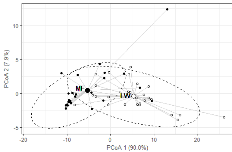
Figure 78: Graphical projection of homogeneity of multivariate dispersions of data around ecosystem type centroids (Principal coordinates analysis). Average distance to centroids were 6.084 and 5.912 for LW and MF, respectively. Small open circles represent plots located in LW sites, small black filled circles correspond to plots located in MF sites. The two big circles represent the group centroids for each forest type (LW vs. MF).
