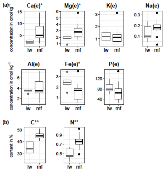
Figure 33: Distributions of chemical compounds in the FH horizon in lichen woodland and moss forest plots (lw and mf, respectively). (a) Concentrations of exchangeable base cations and extractable P, (b) organic C and N. Boxplots represent the distribution around the median values. (e) indicates exchangeable or extractable elements. Asterisks indicate significant difference using mixed models (see Material and Methods), with *: p-value<0.05, **: p-value<0.01, ***: p-value<0.001.
