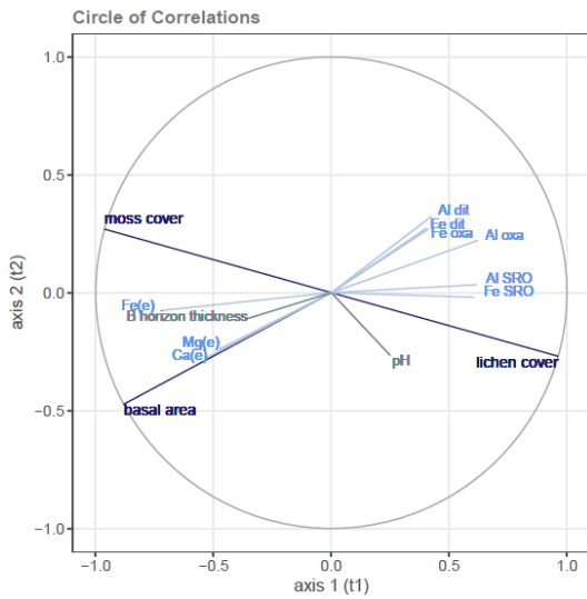
Figure 67: Graphical projection of partial least square canonical analysis (PLSCA) results in the B horizon at the plot scale. Variables for stand tree cover characteristics are drawn in dark blue, chemical compounds are in light blue, and soil characteristics in grey. Axes correspond to principal orthogonal canonical components. Positive, null or negative correlations between variables are indicated by acute, right or obtuse angles, respectively, between the corresponding vectors. (e) indicates exchangeable or extractable elements. Regarding the chemical elements, only variables that showed the greatest differences in mean values between lw and mf plots in the B horizon were included in the PLSCA.
