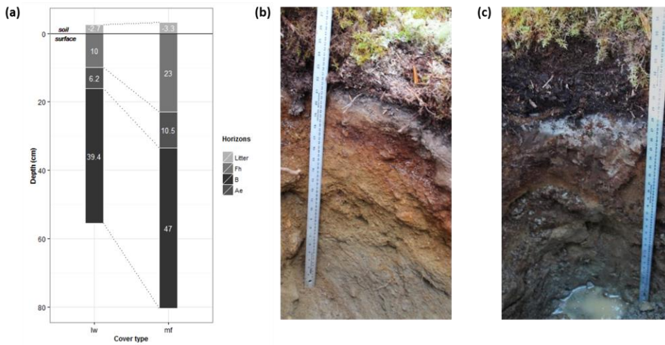
Figure 21: Soil profiles in mf and lw plots. (a) Average thicknesses of the litter, FH, Ae and B horizons. Labels inside stacked bars refer to each horizon's thickness average. (b) Picture taken in the field of a soil profile representative of lw. (c) Picture taken in the field of a soil profile representative of mf. Soil profiles were composed of a thin eluvial pale grey horizon (Ae), a mineral B horizon whose colour varied between sites from light, reddish to dark brown and faded to paler colours with depth, and a grey mineral C horizon.
