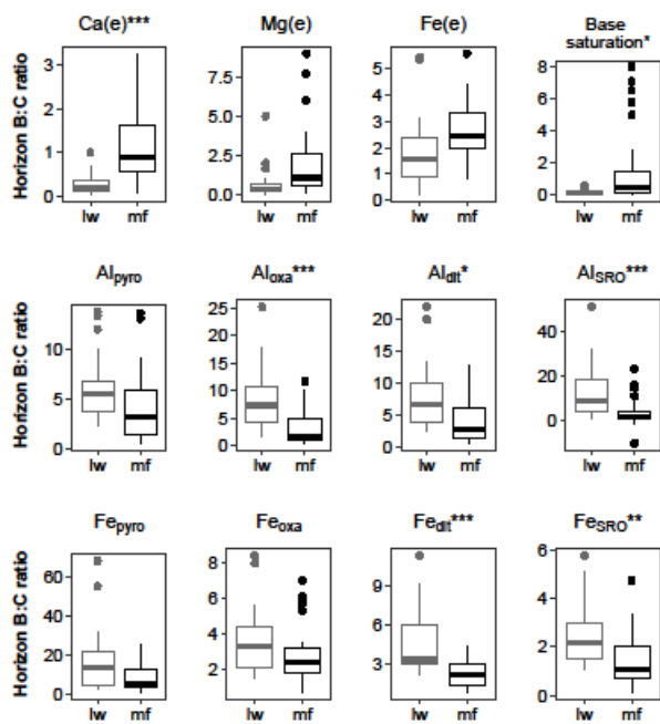
Figure 56: Comparison of horizons B:C ratios in lw and mf plots. Ratios were calculated by dividing for each soil type concentration measured in the B horizon by that measured in the C horizon. (e) indicates exchangeable or extractable elements. "Pyro", "oxa" and "dit" subscripts mention the type of extractions used for isolating Fe and Al species (respectively pyrophosphate, oxalate and dithionite-citrate). "SRO" stand for "short-range order species ( Al_{SRO} = Al_{oxa} - Al_{pyro} , Fe_{SRO} = Fe_{oxa} - Fe_{pyro} ). Asterisks indicate statistical significance using mixed models (see Material and Methods) with *: p-value<0.05, **: p-value<0.01, ***: p-value<0.001.
