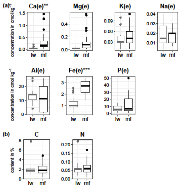
Figure 34: Distribution of chemical compounds in the B horizon in lichen woodland and moss forest plots (lw and mf, respectively). (a) Concentrations of exchangeable base cations and extractable P, (b) organic C and N. Boxplots represent the distribution around the median values. (e) indicates exchangeable or extractable elements. Asterisks indicate significant difference using mixed models (see Material and Methods), with *: p-value<0.05, **: p-value<0.01, ***: p-value<0.001.
