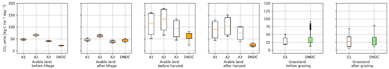
Figure 7: Management effects on CO 2 emissions. Measured and modelled emissions in a time window of 2 weeks before and 2 weeks after a management.
