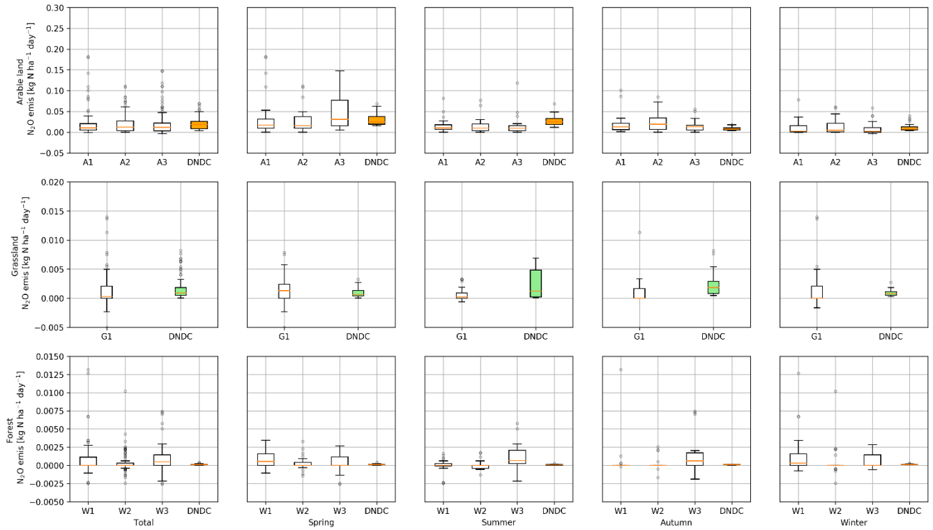
Figure 3: Observed and modelled N 2 O emissions for spring (21 st Mar. - 20 th Jun.), summer (21 st Jun. - 20 th Sep.), autumn (21 st Sep. - 20 th Dec.), and winter (21 st Dec. - 20 th Mar.).
