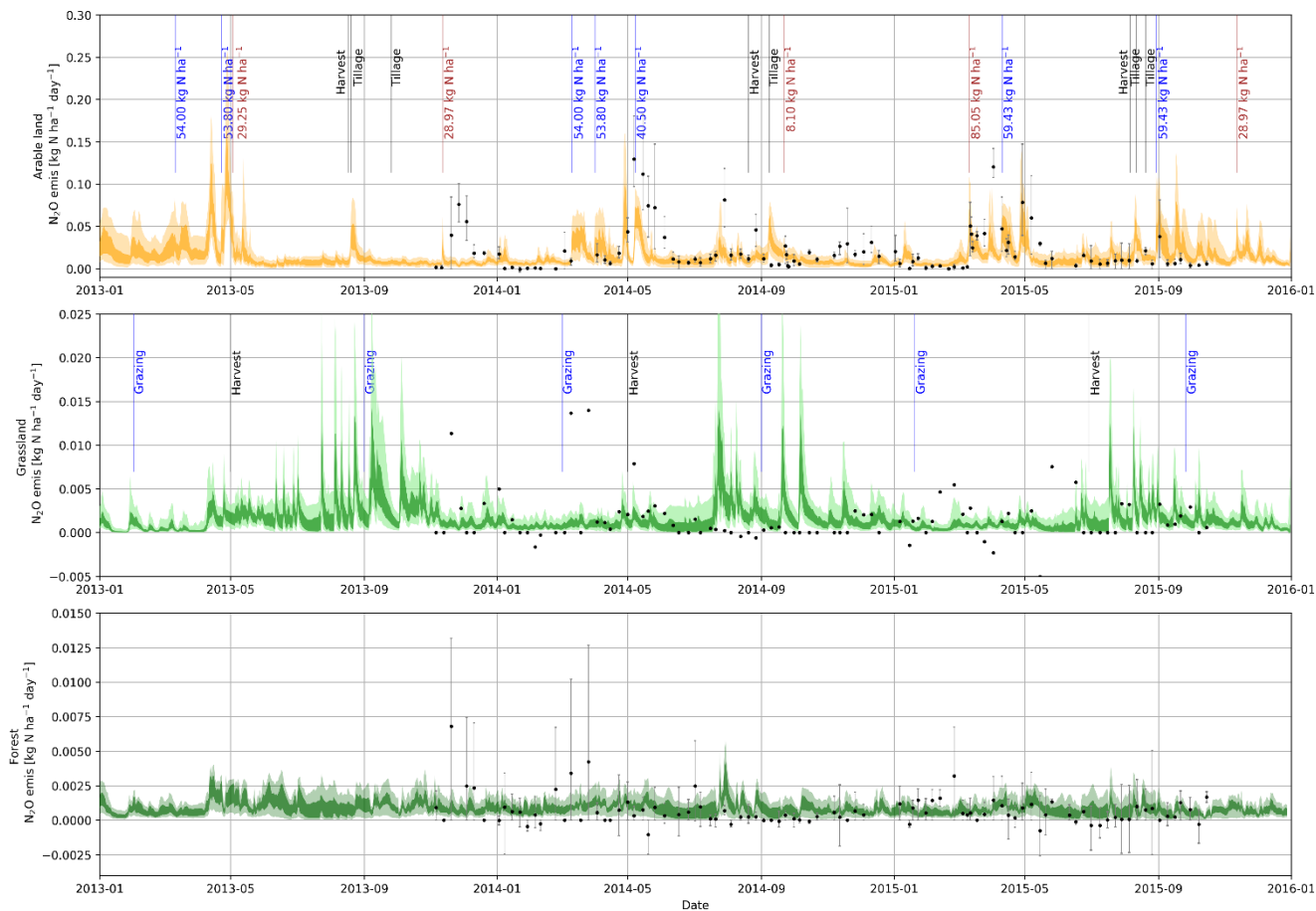
5 Figure 2: Measured and modelled \text{N}_2\text{O} emissions from different land use. Measurements are given as grey error bars showing the variance between the replicated transects and the mean value as a black dot. Posterior model uncertainty is given in light colour for the 5 and 95 percentiles and dark colour for the 25 and 75 percentiles. Vertical lines indicate management events. In the uppermost panel, blue coloured vertical bars indicate fertilizer application, while brown colours indicate manure application.
