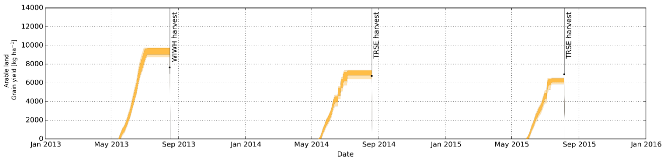
5 Figure A4: Modeled dry weight grain yield on arable land use. WIWH = Winter wheat, TRSE = Triticum secale. RMSEs ranging from 1125.7 to 2529.2 kg ha -1 .
