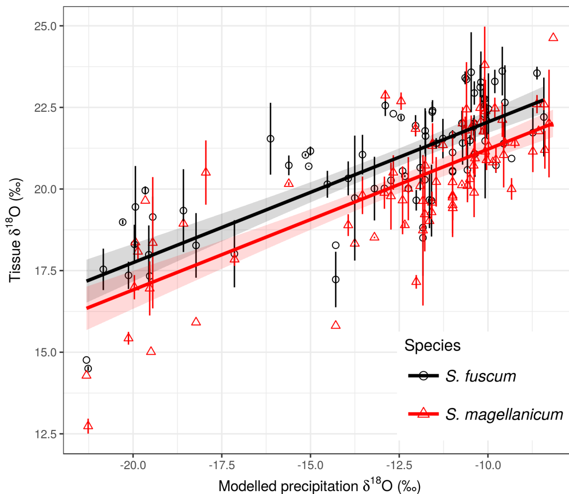
Figure 3. Association between modelled annual mean \delta^{18}\text{O}_{\text{precip}} values and \delta^{18}\text{O} values in two Sphagnum species. Data show predicted-site means for each species and error bars represent the standard deviation (at some sites only one sample of a species was taken BLUPs) and error bars represent the approximate 95% confidence intervals ( 2 \times \text{SE} ). Regression lines with different intercepts ( P < 0.001 , Table 2) illustrate the relationship between modeled \delta^{18}\text{O}_{\text{precip}} and Sphagnum \delta^{18}\text{O} . Equations: S. fuscum , 26.36 + 0.43 \times \delta^{18}\text{O}_{\text{precip}} ( n = 1-2 , N_{\text{site}} = 80 ); S. magellanicum , 25.53 + 0.43 \times \delta^{18}\text{O}_{\text{precip}} ( n = 1-2 , N_{\text{site}} = 83 ). Shaded areas indicate approximate 95% confidence intervals ( 2 \times \text{SE} ) of the regression coefficients that do not include the uncertainty of the random effects.
