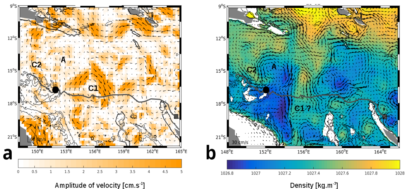
Figure 5. (a) Amplitude of surface geostrophic velocity on February 29th during O2, 2016 calculated from AVISO product ; (b) Density and velocity field at 300 m depth on February 29th during O2, 2016 calculated from HYCOM re-analysis. The gray line corresponds to the full trajectory of float 656 and the black point to the location of the float at the stated date. The black lines correspond to the bottom topography with 300 m and 1000 m depth.
