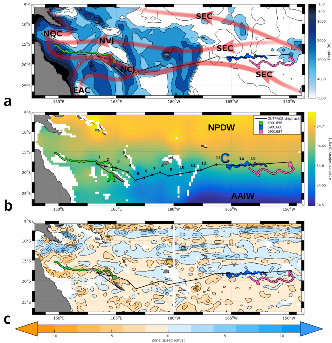
Figure 1. South-west Pacific Ocean (a) main trajectories of zonal jets superimposed on the bottom topography (in m), (b) absolute salinity ( \text{g.kg}^{-1} ) at 1000 m for November climatology from the ISAS13 atlas and (c) zonal mean current (in \text{cm/s} , positive for eastward velocity) deduced from the Argo float displacement at their parking depth (near 1000 m, adapted from Ollivault and Colin de Verdière, 2014). The colored lines represent the studied floats (WMO number in the inset) with squares for their immersion location. The currents shown in the upper panel are the South Equatorial Current (SEC), the North Vanuatu Jet (NVJ), the North Caledonia Jet (NCJ), the North Queensland Current (NQC) and the East Australia Current (EAC). The water masses shown on the middle panel are the North Pacific Deep Water (NPDW) and the Antarctic Intermediate Waters (AAIW). The black line represents the shiptrack of the OUTPACE cruise and, in the middle panel, the crosses represent the short time stations (numbers) and the squares A and C represent two the long time stations of the cruise where the floats in this study were deployed.
