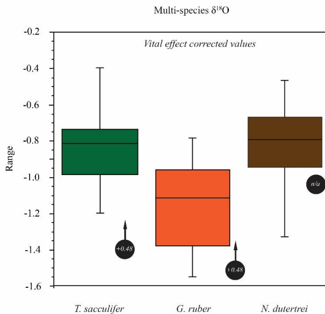
10 Figure 6: Box-plots of the oxygen isotope values ( \delta^{18}\text{O} ) versus size and for different species of planktonic foraminifera. (A) Small, medium and large (see text for definition of sizes represented, note uneven size interval). (B) The (right hand side) box-plots are the range in oxygen isotopes corrected for vital effects (circles with arrows) calculated from in situ water sampling (plankton pump and plankton tow; Peeters data unpublished). The central bar of each box represents the Median.
