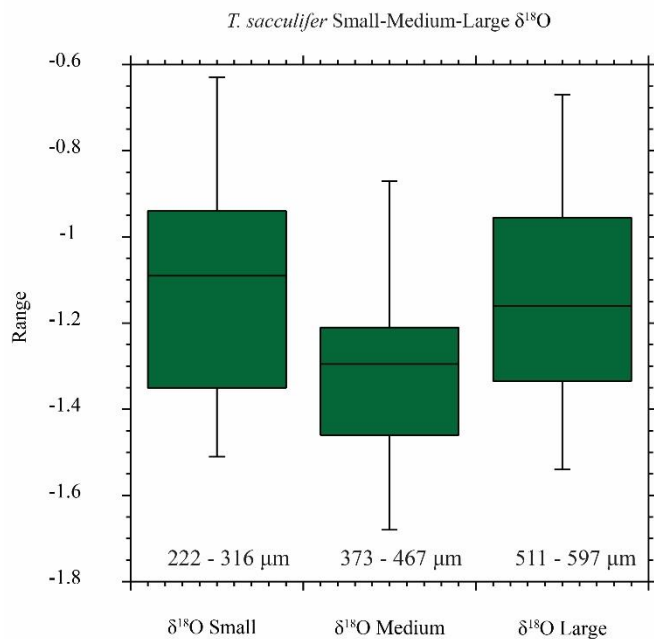
10 Figure 6: Box-plots of the oxygen isotope values ( \delta^{18}\text{O} ) versus size and for different species of planktonic foraminifera. (A) Small, medium and large (see text for definition of sizes represented, note uneven size interval). (B) The (right hand side) box-plots are the range in oxygen isotopes corrected for vital effects (circles with arrows) calculated from in situ water sampling (plankton pump and plankton tow; Peeters data unpublished). The central bar of each box represents the Median.
