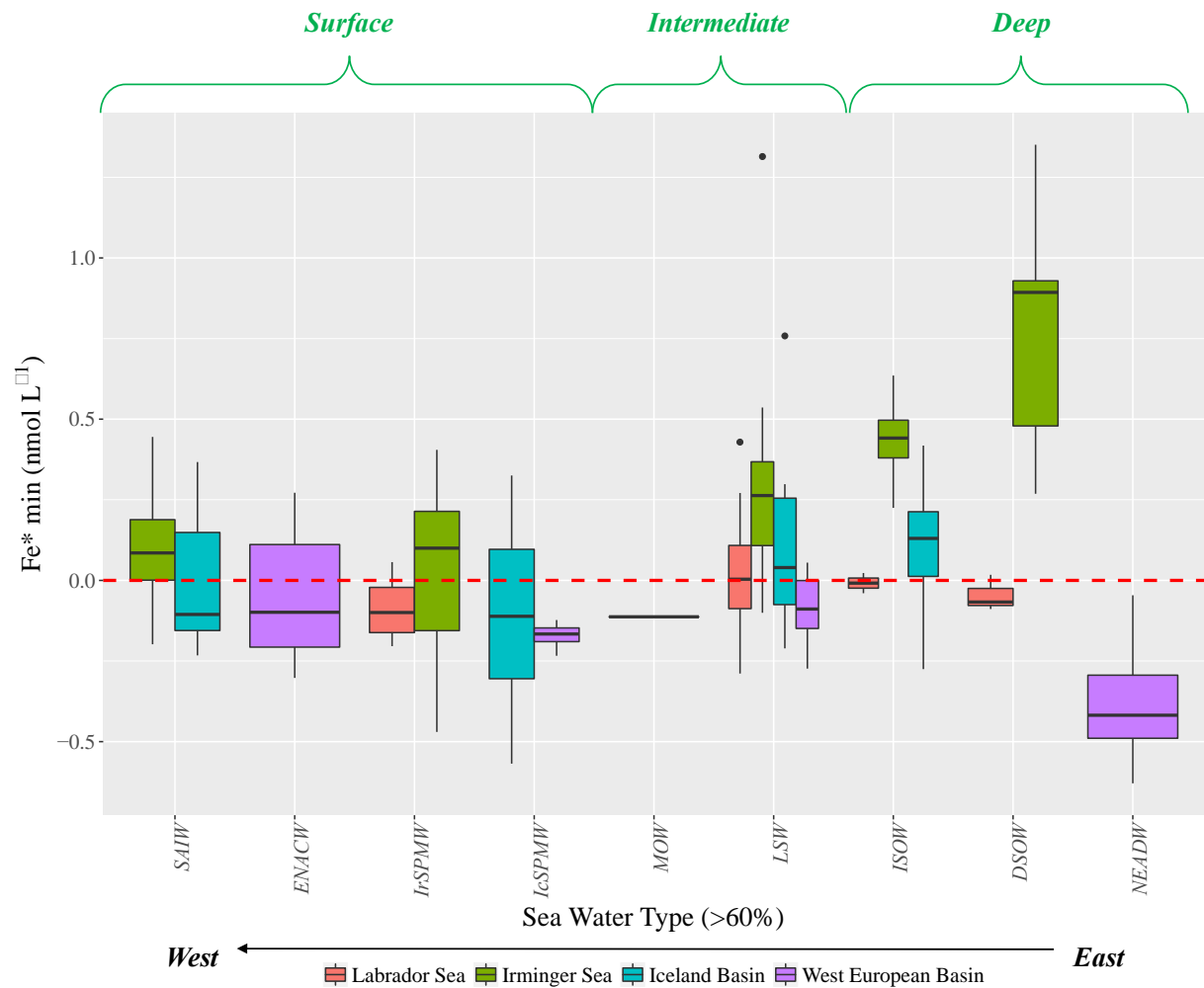
Figure S10: Box and whisker plot of \text{Fe}^* in units of \text{nmol L}^{-1} as determined per water mass and basin with a Fe:N uptake rate of 0.05. Color coding representing from West to East, the Labrador Sea (red), the Irminger Sea (green), the Iceland Basin (blue) and the West European Basin (purple). Abbreviation referring to SAIW: Sub-Arctic Intermediate Water, ENACW: East North Atlantic Central Water, IrSPMW: Irminger Sub-Polar Mode Water, IcSPMW: Iceland Sub-Polar Mode Water, MOW: Mediterranean Overflow Water, LSW: Labrador Sea Water, ISOW: Iceland-Scotland Overflow Water, DSOW: Denmark Strait Overflow Water, NEADW: North East Atlantic Deep Water.
