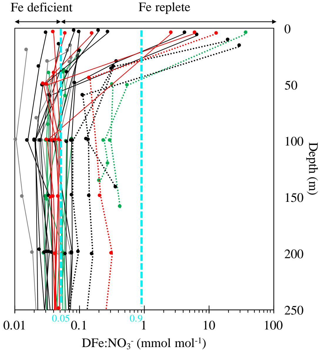
5 Figure S7: Vertical profiles of the \text{DFe:NO}_3^- ratio over the upper 200 m of the water column along the GEOVIDE section. Profiles from the West European Basin are plotted in black, from the Iceland Basin in grey, from the Irminger Sea in green and from the Labrador Sea in red. Stations located above the continental Plateau (stations 1, 2 and 4 from the Iberian Margin; stations 53 and 61 from the Greenland shelf; station 78 from the Newfoundland Margin) are represented with dotted lines. The vertical dashed lines (light blue) indicate lower and upper limits of phytoplankton cellular \text{DFe:NO}_3^- ratios under Fe replete conditions Ho et al., 2003; Sunda and Huntsman, 1995; Twining et al., 2004.
