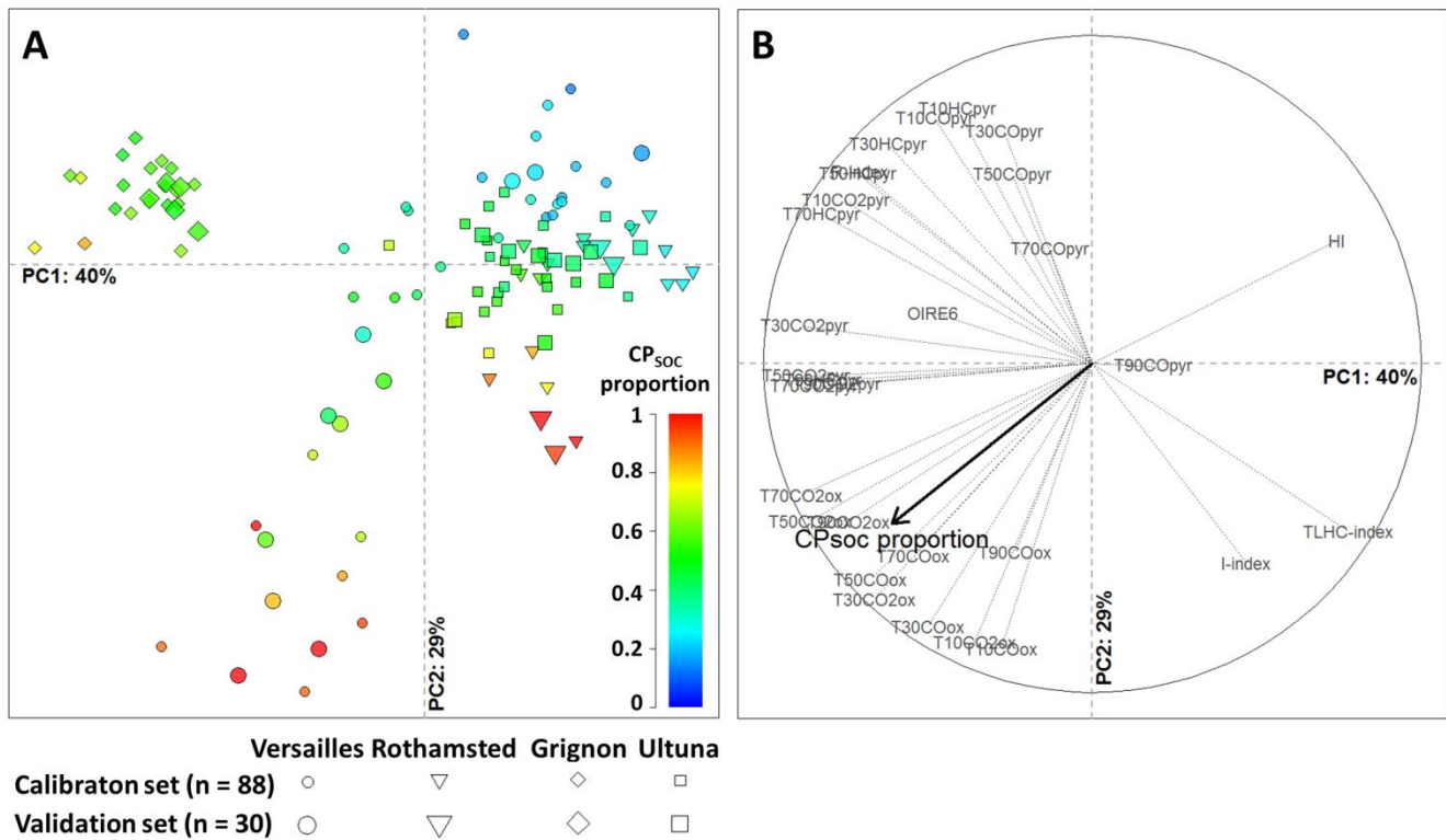
5 | Figure 3: Principal component analysis (PCA) of the 30 RE6 parameters of the calibration soil-sample set with soils from all sites (n = 88). A: the scores of the calibration samples on the first two principal components are represented in the factorial map, as well as the projected principal component scores of the validation samples (n = 30; with soils from all sites ). A color scale is used to represent the CP SOC proportion (determined using Eq. (2)) in all samples. B: PCA loadings of the 30 RE6 parameters and projection of the CP SOC proportion variable in the PCA correlation circle. Note that despite some of the 30 RE6 parameters are significantly correlated, all parameters are included in the analysis.
