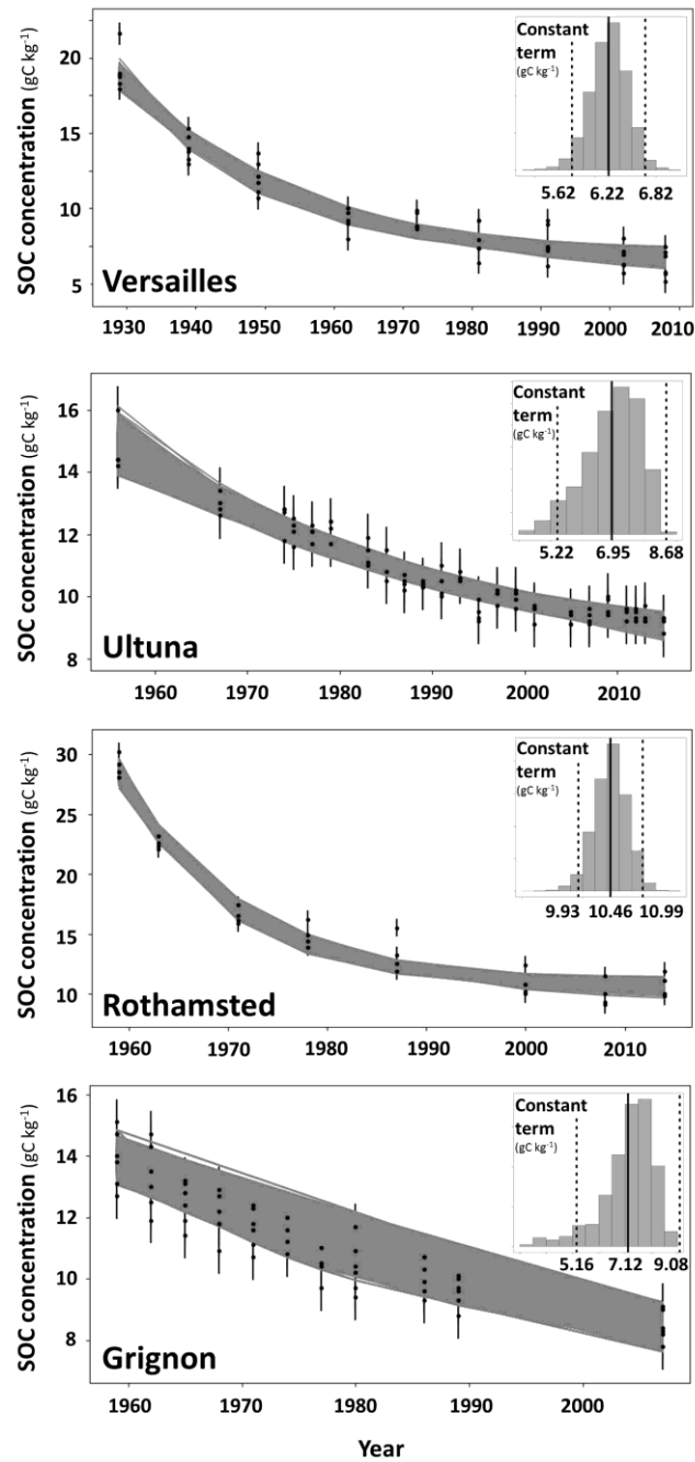
5 Figure 2: Evolution of SOC concentration ( \text{gC.kg}^{-1} soil) with time for the bare fallow plots of each experimental site, and representation of the 3 \times 10^4 fitted exponential decay functions (Bayesian curve fitting method) from which a site-specific \text{CP}_{\text{SOC}} concentration (model parameter c ) and its 95% confidence interval were determined (histogram in the upper right side of each scatter plot). At each site, the 95% confidence interval around the \text{CP}_{\text{SOC}} concentration was determined as c \pm 1.96 \text{sd}(c) , where c is the model parameter c in Eq. (1) and \text{sd}(c) is its standard deviation.
