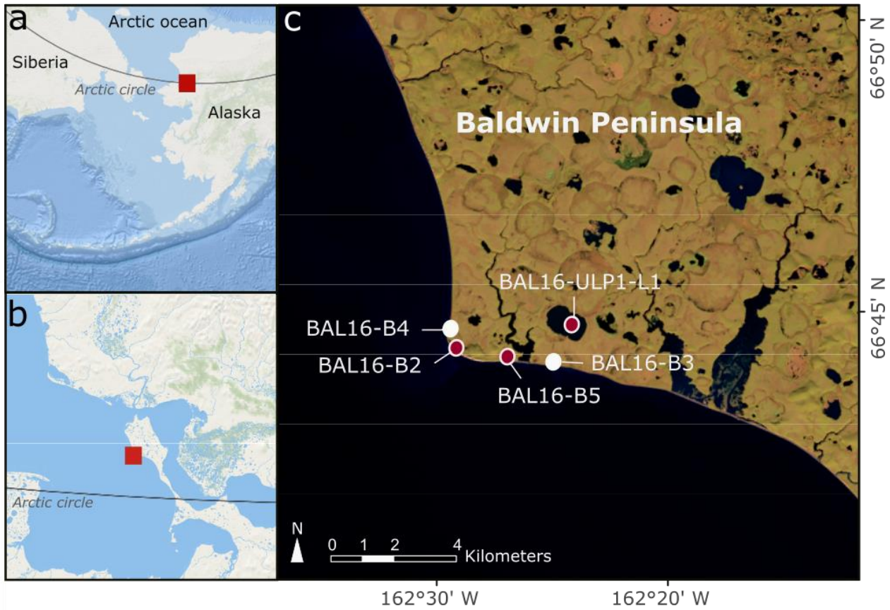
5 Figure 1: (a) Overview map of Siberia and Alaska with indicated study region (red square). (b) Close-up of Kotzebue Sound with indicated study region (red square). (c) Study sites on Baldwin Peninsula presented in this study (purple filled dots) and additional sites used in the organic carbon pool calculations (white dots); false color image with short-wave infrared, near-infrared and deep blue bands (7-5-1). Source for background map in (a) and (b): World Ocean Base (ESRI); satellite image map (c): Landsat 8 image from 13 Oct. 2016, USGS/NASA.
