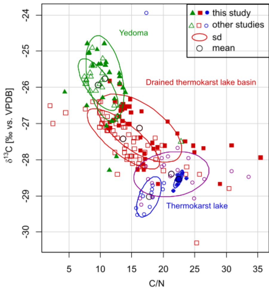
5 Figure 5: Scatterplot of total organic carbon-total nitrogen (C/N) ratio and stable carbon isotopes ( \delta^{13}\text{C} ) of yedoma deposits (green triangles), drained thermokarst lake basin (DTLB) deposits (red squares) and thermokarst lake sediments (blue and purple dots) in Alaska. Mean value and standard deviation (sd) indicated. Data from this study (filled symbols): Baldwin Peninsula; data from other studies (hollow symbols): Itkillik River (Lapointe et al., 2017; Strauss et al., 2012), Northern Seward Peninsula (Lenz et al., 2016a) and lakes from Kobuk River Delta (blue) and Central Seward Peninsula (purple) (Lenz et al., 2018).
