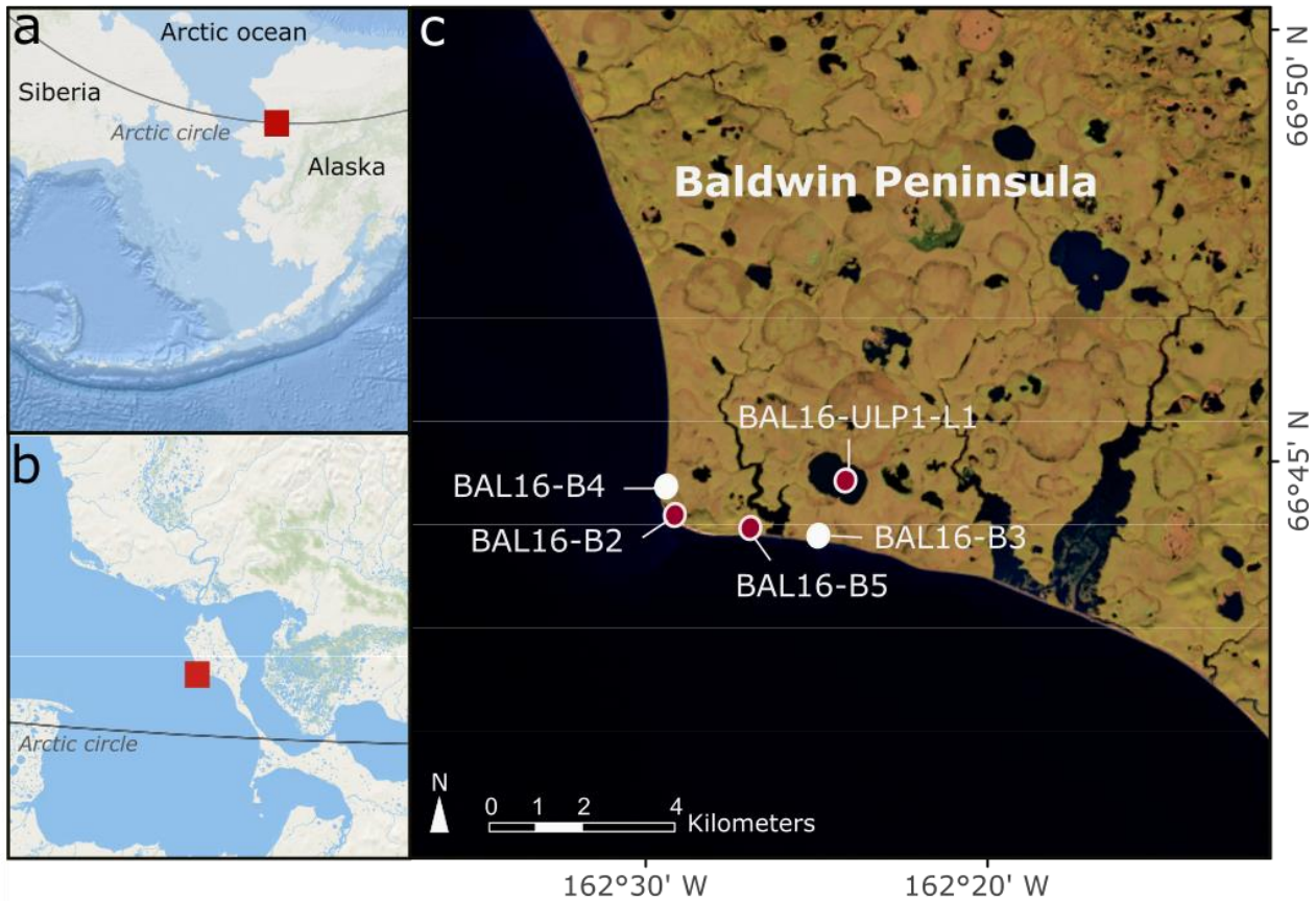
Figure 1: (a) Overview map of Siberia and Alaska with indicated study region (red square). (b) Close-up of Kotzebue Sound with indicated study region (red square). (c) Study sites on Baldwin Peninsula presented in this study (purple filled dots) and additional sites used in the organic carbon pool calculations (white dots); false color image with short-wave infrared, near-infrared and deep blue bands (7-5-1). Source for background map in (a) and (b): World Ocean Base (ESRI); satellite image map (c): Landsat 8 image from 13 Oct. 2016, USGS/NASA.
