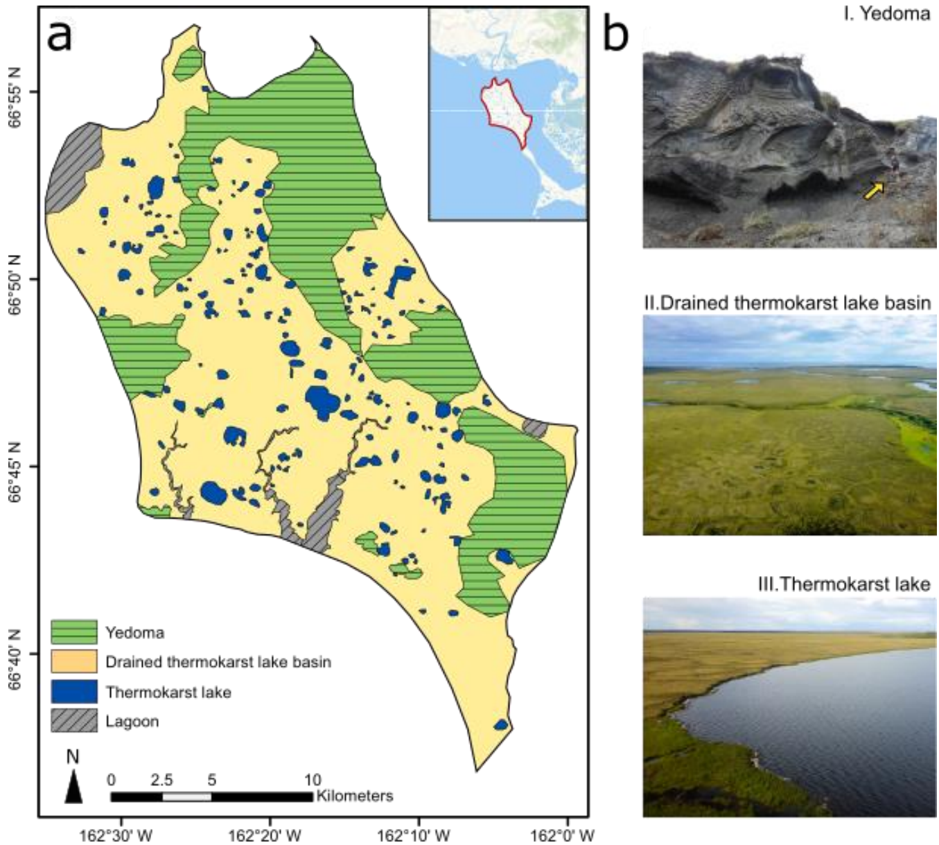
5 Figure 4: a) Land cover classification map of Baldwin Peninsula (see overview map in upper-right corner) with yedoma (green), drained thermokarst lake basins (yellow), thermokarst lakes (blue) and lagoons (grey). B) Exemplary photos: I. Yedoma (note person on the right indicated by yellow arrow for scale), II. Drained thermokarst lake basin and III. Thermokarst lake. Source for overview map in (a): World Ocean Base (ESRI).
