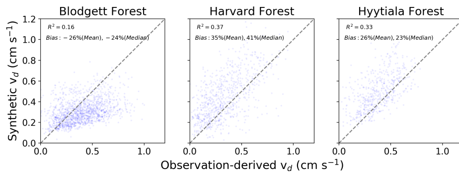
Fig. 2. Synthetic and observation-derived daily daytime O 3 deposition velocity.
