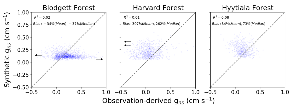
Fig. 1. Synthetic and observation-derived daily daytime O 3 non-stomatal conductance
