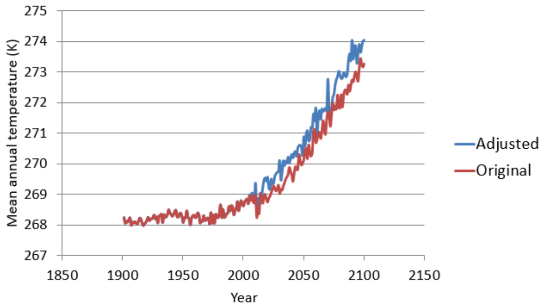
Fig. 1. Fig. R1 Global mean annual temperature changes from 1901 to 2100. Historical data were interpolated from 6-hourly (Qian et al., 2006) to hourly and re-gridded from a spatial resolution of 0.5° by 0.5°
