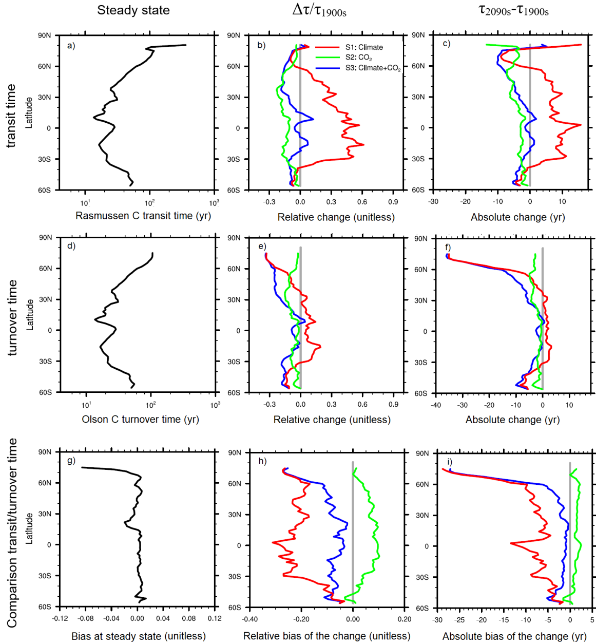
Figure 6 a) Latitudinal variation in C transit time ( \tau_{Rts} ) at steady state and b)-c) its change are compared to d)-f) C turnover time ( \tau_{eto} ). The changes between 2090s and 1900s are estimated by c), f) absolute value: \Delta\tau = (\tau_{2090s} - \tau_{1900s}) and by b), e) relative value: \Delta\tau_r = \frac{\Delta\tau}{\tau_{1900s}} . g) The biasdeviation of C turnover time in relative to C transit time is estimated by (\tau_{eto} - \tau_{Rts})/\tau_{ts} at steady state. In relative to C transit time, the biasdeviation of the change in C turnover time are estimated by h) absolute biasdeviation ( |\Delta\tau_{eto}| - |\Delta\tau_{Rts}| ) and i) relative biasdeviation in \frac{(|\Delta\tau_{eto}| - |\Delta\tau_{Rts}|)}{|\Delta\tau_{Rts}|} . All variables are compared in three scenarios: S1: only climate warming scenario (red line); S2: rising atmospheric [CO 2 ] scenario (green line), and S3: Combination of climate warming and rising atmospheric [CO 2 ] scenario (blue line). Grey lines in b), c), e) and f) represent the reference lines of no change and those in h) and i) represent reference line of no biasdeviation .
