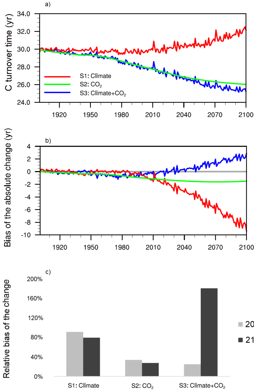
Figure 5 a) Changes of global C turnover time (stock-over-flux) in three scenarios, S1: climate warming scenario (red line); S2: rising atmospheric [CO 2 ] scenario (green line), and S3: Combination of climate warming and rising atmospheric [CO 2 ] scenario (blue line). b) The biasdeviation of the change in C turnover time ( \Delta\tau_{eto} ) is estimated relative to the change in C transit time ( \Delta\tau_{Rts} ): (|\Delta\tau_{eto}| - |\Delta\tau_{Rts}|) . Positive indicates more change in C turnover time than C transit time. Grey line represents the reference of no biasdeviation . c) The relative biasdeviation of the change in C turnover time in year 2000 and 2100 is also estimated relative to the change in C transit time: \frac{(|\Delta\tau_{eto}| - |\Delta\tau_{Rts}|)}{|\Delta\tau_{Rts}|} \times 100\% .
