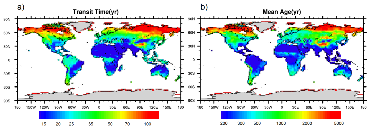
Figure 1 Global maps of a) carbon transit time and b) carbon mean age are the average over 1901 to 1910 at each grid cell.
