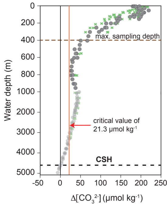
Figure 4. Calcite saturation state indicated by \Delta[\text{CO}_3^{2-}] depth profiles of the Caribbean Sea and Gulf of Mexico. Grey dots and green crosses: Transect A22 (stations 10–15) and NACPECC (stations 20–28) (Fig. 1) with \Delta[\text{CO}_3^{2-}] being the difference between [\text{CO}_3^{2-}]_{\text{in-situ}} and [\text{CO}_3^{2-}]_{\text{saturation}} . Alkalinity and \text{TCO}_2 were taken from WOCE and NACP (cchdo.ucsd.edu; cruise RV Knorr in 1997, EXPOCODE: 316N151_4 and cruise RV Ronald H. Brown in 2007, EXPOCODE: 33RO20070710) to calculate [\text{CO}_3^{2-}]_{\text{in-situ}} using the program CO2SYS (Pierrot et al., 2006; taking the constants ( K_1 and K_2 ) of Mehrbach et al. (1973) refitted by Dickson and Millero (1987) and ( K_{\text{SO}_4} ) from Dickson (1990)). [\text{CO}_3^{2-}]_{\text{saturation}} was calculated after Jansen et al. (2002). Red vertical line indicates the critical \Delta[\text{CO}_3^{2-}] value of 21.3 \mu\text{mol kg}^{-1} below which selective \text{Mg}^{2+} ion removal starts (Regenberg et al., 2014); black dashed line marks the calcite saturation horizon (CSH), which is defined to 0 \mu\text{mol kg}^{-1} and represents the top of the lysocline at \sim 4600 m water depth; brown dashed line indicates the maximum plankton tow sampling depth.
