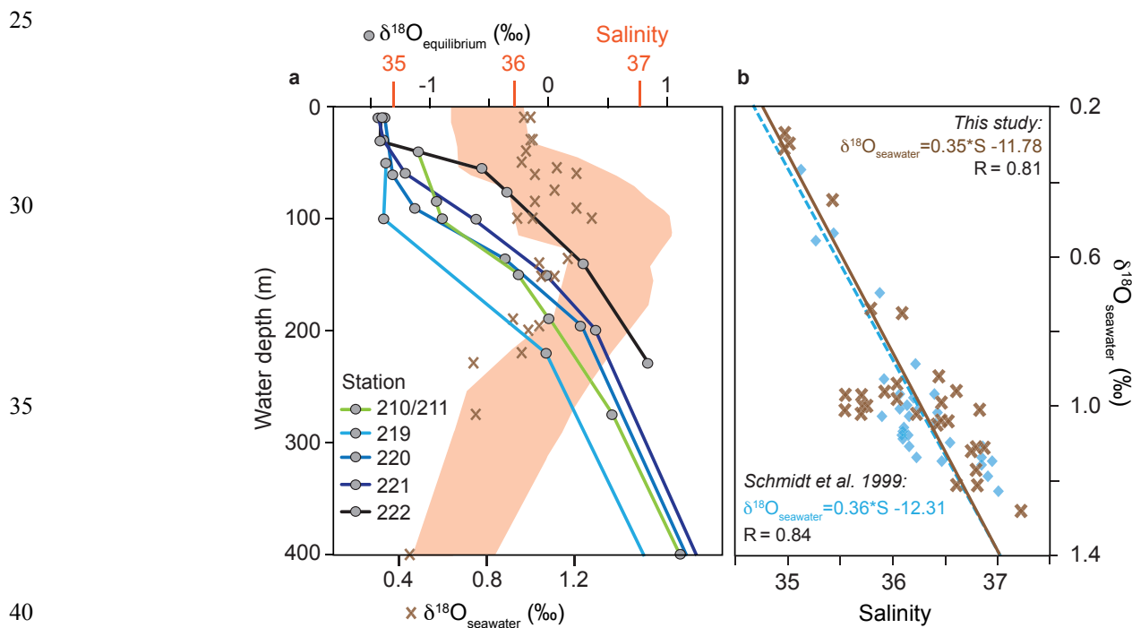
Figure 3. a) \delta^{18}\text{O}_{\text{seawater}} (‰ VSMOW) and colour-coded \delta^{18}\text{O}_{\text{equilibrium}} (‰ PDB) depth profiles at the CTD stations 210/211, 219, 220, 221, and 222 (see Fig. 1). Red shading: Salinity envelope of the ambient seawater from Florida Straits and Caribbean Sea measured during cruise M78/1 matching \delta^{18}\text{O}_{\text{seawater}} . b) Brown crosses: Measured in situ salinity vs.
