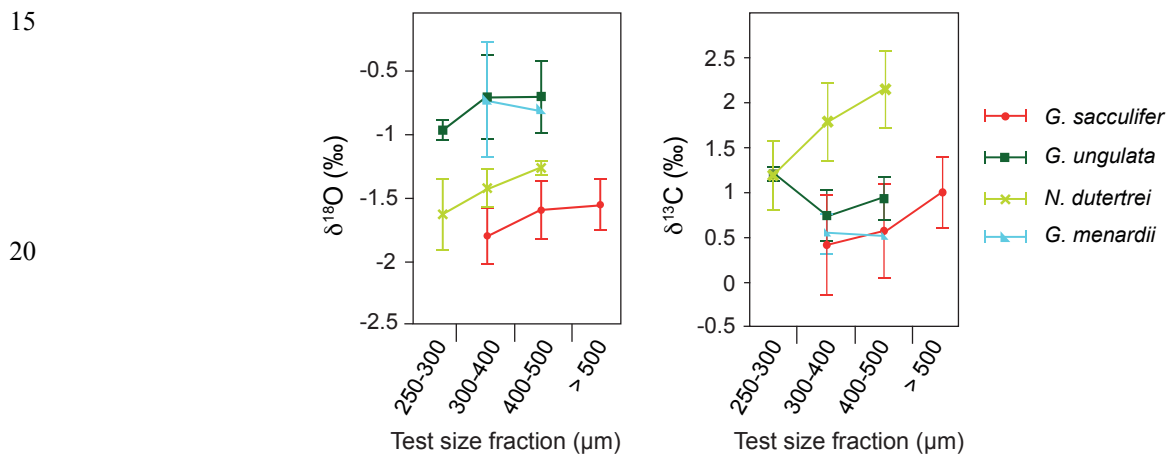
Figure 5. Stable oxygen and carbon isotopes (average \delta^{18}\text{O}_{\text{calcite}} and \delta^{13}\text{C}_{\text{calcite}} \pm standard deviations) compared to different test size fractions of living planktic foraminifers (only species with more than one analysed test size fractions are depicted).
