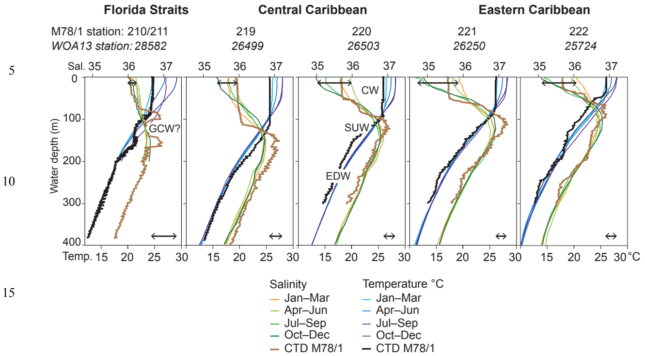
Figure 2. Temperature ( ^{\circ}\text{C} ) and salinity depth profiles in the working area. In situ CTD data measured during cruise M78/1 (March 2009, thick brown and black lines) are presented in comparison to the seasonally differentiated World Ocean Atlas 2013 (WOA13) data (Locarnini et al., 2013; Zweng et al., 2013; coloured thin lines). GCW: Gulf Common Water; CW: Caribbean Water; SUW: Subtropical Under Water; EDW: 18^{\circ}\text{C} Sargasso Sea Water. Black double arrows indicate the seasonal ranges of temperature (bottom) and salinity (top) in the uppermost water column (0–10 m water depth).
