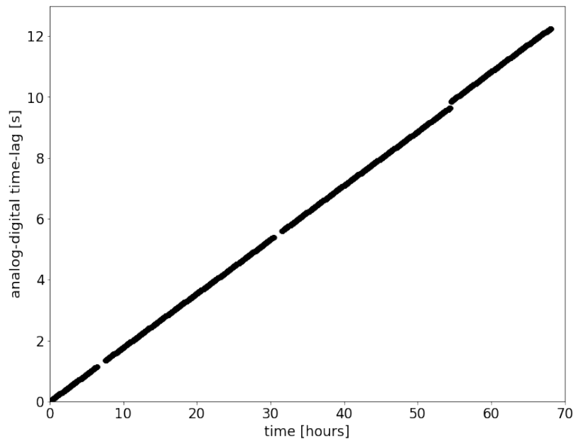
5 Figure 9: Evolution of time-lags between two replicates of the same variable ( u wind component, but identical results were obtained with v and w ), one collected with the SAT native digital format and one collected via analog outputs from the SAT. Data were collected in two files roughly 70 hours long and then split into 30-min chunks for the computation of time-lags.
