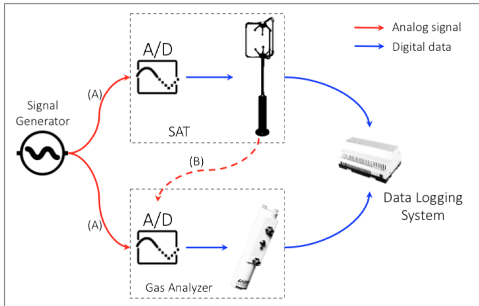
5 Figure 8: Schematic of possible setups to evaluate the ability of a data logging system to synchronise EC data. In setup A the same (known) analog signal (solid red lines) is sent to the analog inputs of the EC instruments where it is digitized. In setup B analog wind data (dashed red line) is sent to the gas analyser, where it is digitized. In both setups, the 2 digital data streams are then collected by the data logging system. The clocks involved and how timestamps are attached to data depend on the specifics of the system under consideration.
