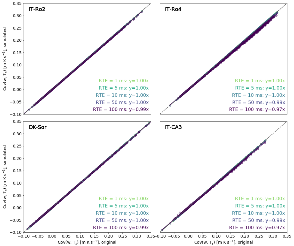
Figure 4: Simulation of RTEs. Covariances w-T_s obtained with a set of simulated random errors of different amplitudes (y-axes) are compared to the covariances w-T_s computed with the original time series (x-axes), for the four sites. All regressions had offset equal to zero and r^2 > 0.99 .
