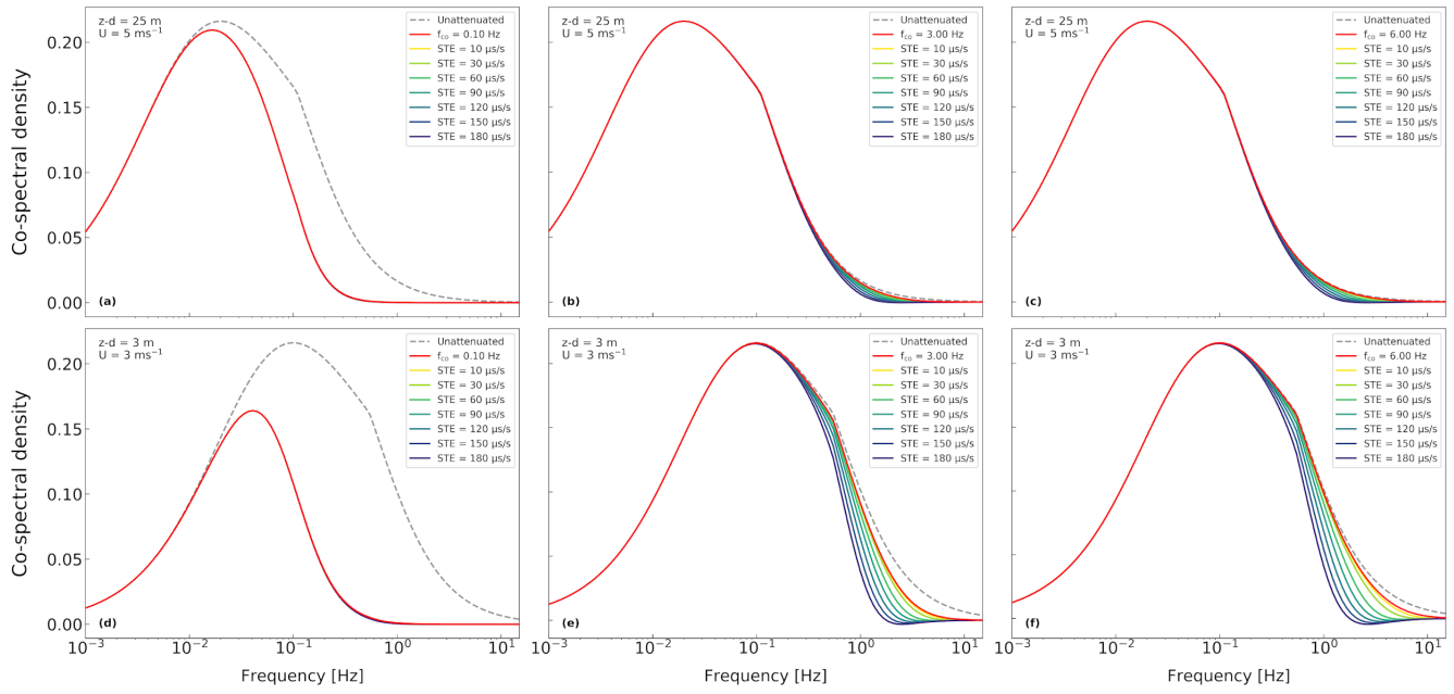
5 Figure 7: Effect of adding artificial STEs to three EC systems characterized by different cutoff frequencies (0.1, 3.0 and 6.0 Hz, from left to right) and by different measurement height and mean wind speed (top to bottom).
