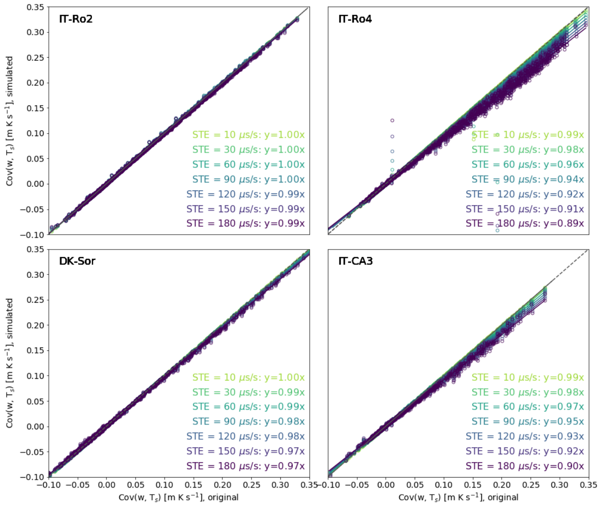
Figure 5: Simulation of STE. Covariances w-T_s obtained with a set of simulated systematic errors of different amplitudes (y-axes) are compared to the covariances w-T_s computed with the original time series (x-axes), for the four sites. All regressions had offset equal to zero and r^2 > 0.98 .
