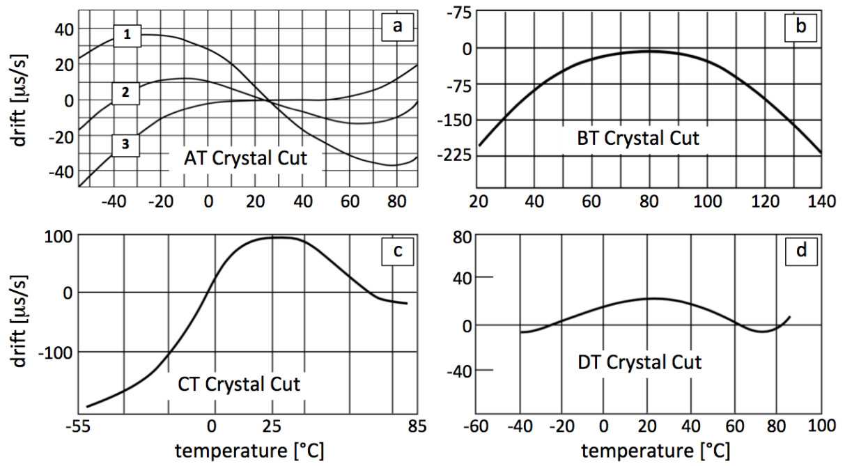
5 Figure 2: Exemplary temperature dependence curves for clocks with AT (a), BT (b), CT (c) and DT (d) cuts. In (a) the 3 curves refer to different angles of rotations of the crystal. Reproduced and adjusted from Hewlett Packard (1997).
