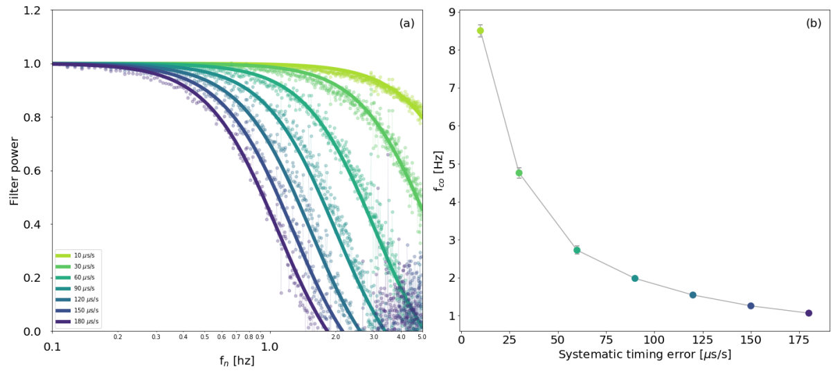
5 Figure 6: Transfer function for the STE at different error amounts, as derived using Eqs. 2 and 3, using data from site IT-CA3 (a). Mean values and 3.5 \sigma ranges of the transfer function cutoff frequencies across the four sites, as a function of the error amount (b).
