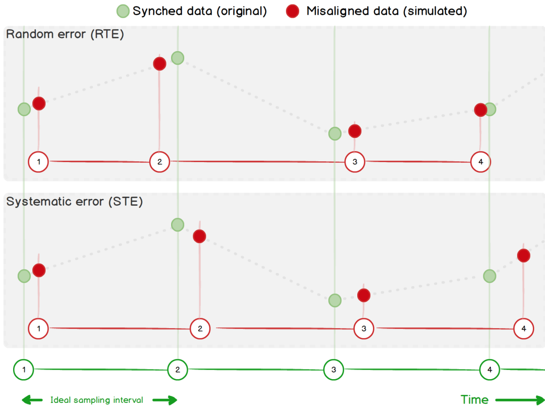
5 Figure 3: Sketch of the timing error simulation via linear interpolation. Green dots represent original T_s data points, equally spaced at the prescribed (nominal) time steps. In the upper panel, RTEs are simulated as time steps randomly varying around the nominal value. In the lower panel, STEs are simulated as a time step larger than the nominal one, whereby the difference between the assigned and correct timestamps always increase in time.
