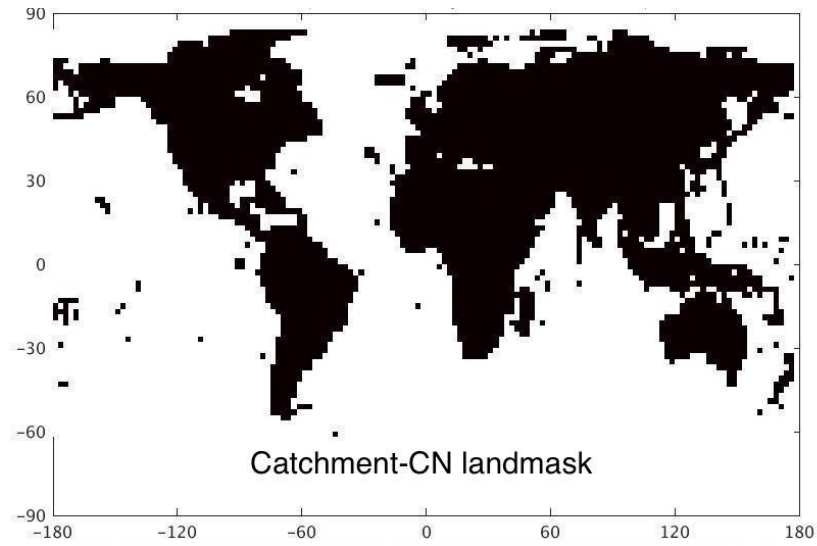
Figure L2a. Landmask of Catchment-CN (previous)
