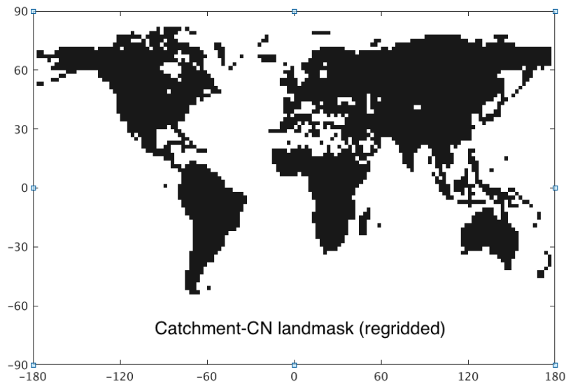
Figure L2b. Landmask of Catchment-CN (regridded)
