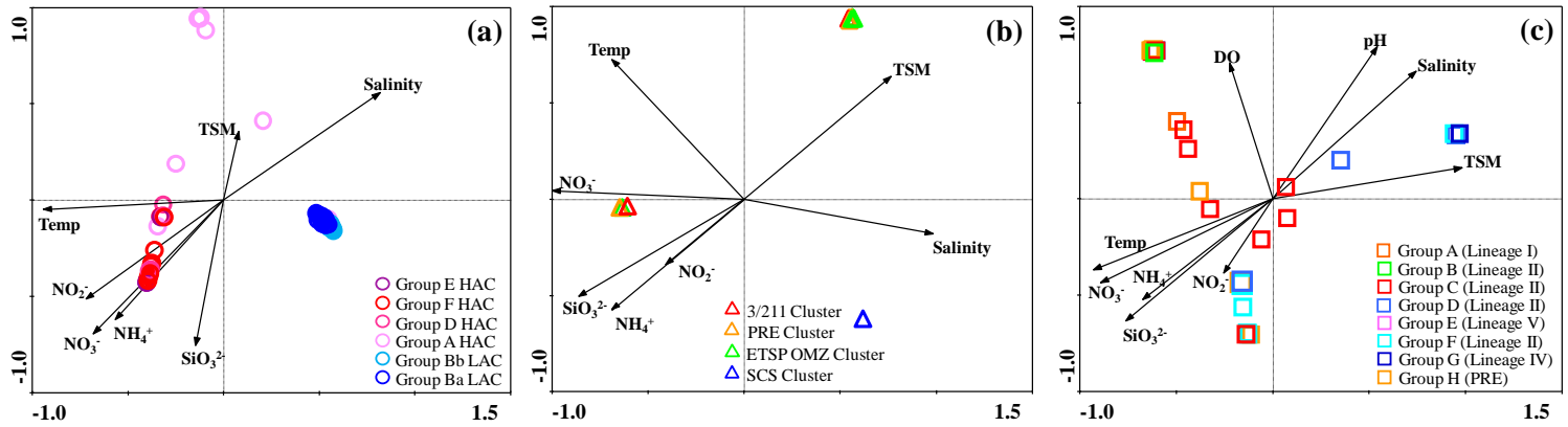
1 2 Figure 10. Canonical correspondence analysis (CCA). (a) Ammonia-oxidizing archaea, (b) Nitrospina , and (c) 3 Nitrospira phylogenetic taxa under the constraint of environmental factors. Each symbol represents an individual OTU. 4 Vectors represent the environmental variables. Temp, temperature. DO and pH were not included in (a) and (b) because 5 they were not measured at SEATS.
