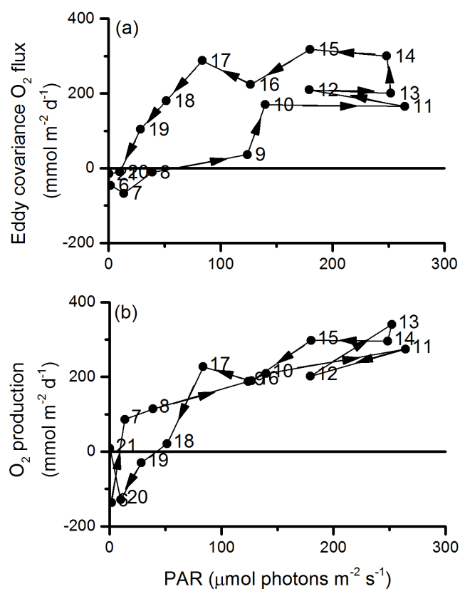
Figure 2. Diurnal hysteresis in oxygen flux at the open-water seagrass meadow. Eddy covariance O 2 fluxes measured above the meadow as a function of irradiance (a). O 2 fluxes corrected to account for O 2 concentration change (i.e. storage) in the water between the eddy covariance measurement volume and the sediment, including the meadow (b). Labels represent the hour of the day.
