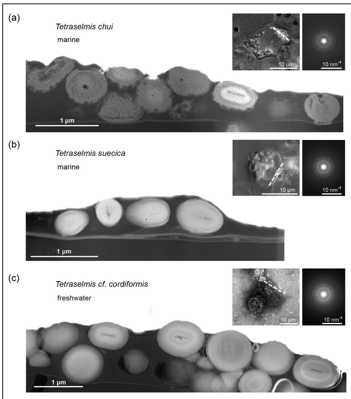
5 Figure 2: Comparison of FIB-cut sections of cells of three different Tetraselmis species (dried samples).
