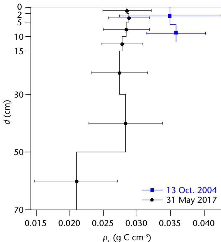
Figure 3. Average soil carbon density ( \rho_c ) for seven different depth layers between the surface on 13 October 2004 and a depth of d = 70 cm (31 May 2017). Error bars show standard deviations.
