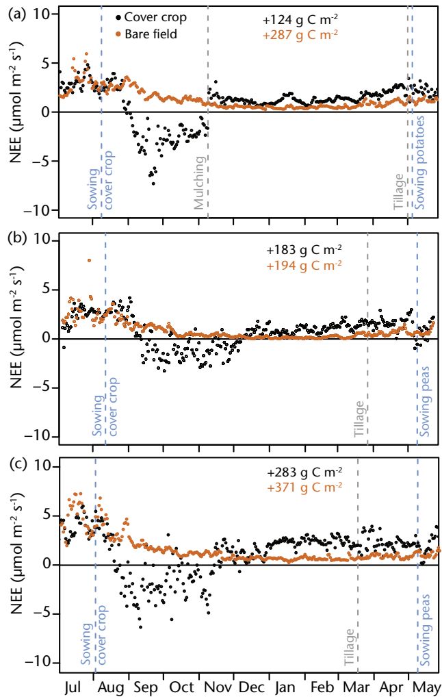
Figure 5. Daily average NEE of the three cover crop seasons: (a) 2005/2006, (b) 2009/2010 and (c) 2015/2016 displaying measured data with cover crop and modelled data with a bare field. Measured-NEE was measured with an EC system while modelled NEE was simulated with the model SPA-Crop. Vertical lines indicate sowing, tillage and mulching dates. Numbers in the top right corner of each subfigure are cumulative NEE of the field with cover crop in black and of the bare field in brown.
