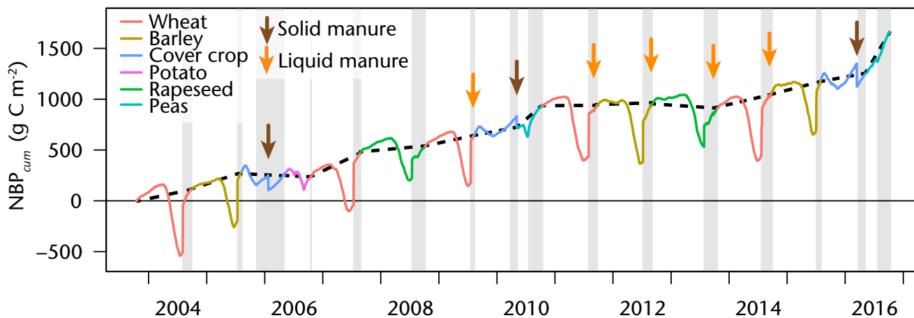
Figure 2. Daily cumulative net biome production ( \text{NBP}_{cum} ) between 16 Oct 2003 and 11 Oct 2016. The black dashed line connects \text{NBP}_{cum} at the end of each crop season. During time periods with a grey background, the field was bare (from harvest of a crop to sowing of the next crop or from first ploughing after sowing of a crop to sowing of the next crop if the first crop was not harvested).
