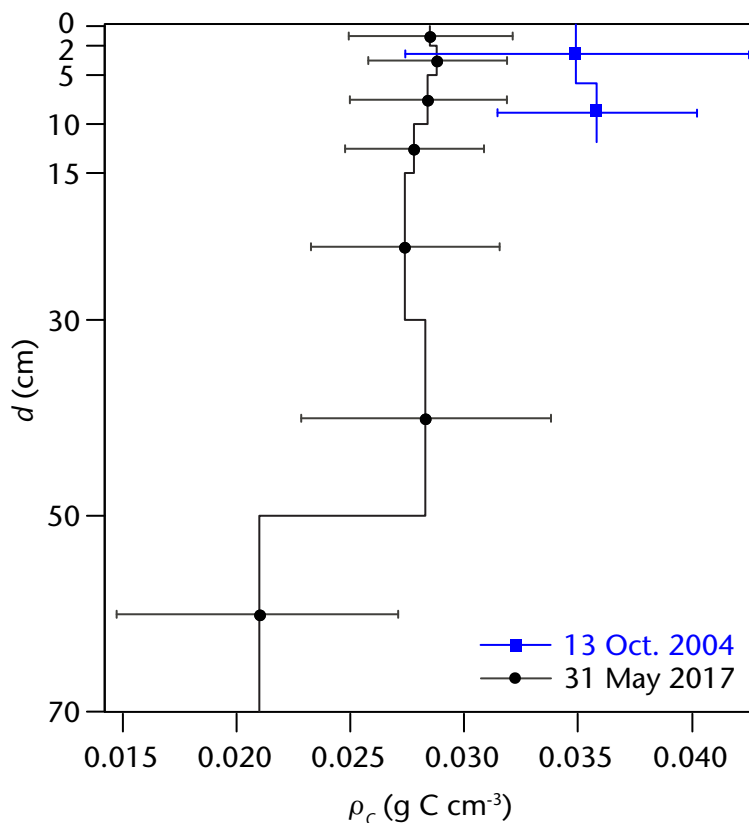
Figure 3. Average soil carbon density ( \rho_C ) for different depth layers on 13 October 2004 and 31 May 2017. Error bars show standard deviations.
