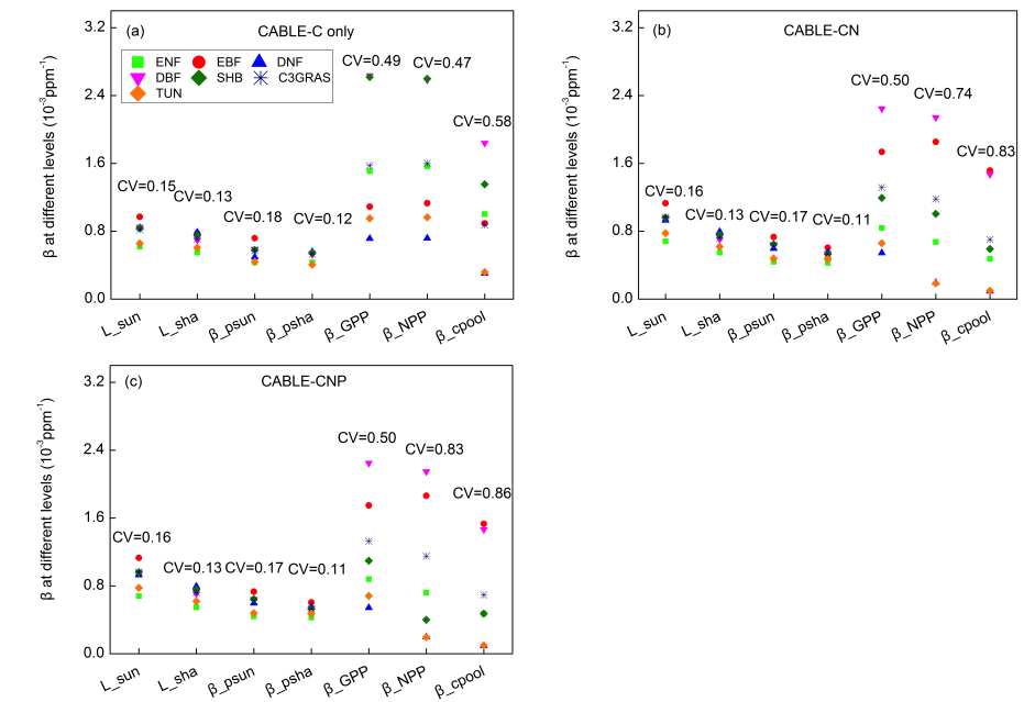
Fig. 1. \beta values at different levels for various C3 plants at the year 2023 from CABLE-C only(a), CABLE-CN (b) and CABLE-CNP (c) simulations.
