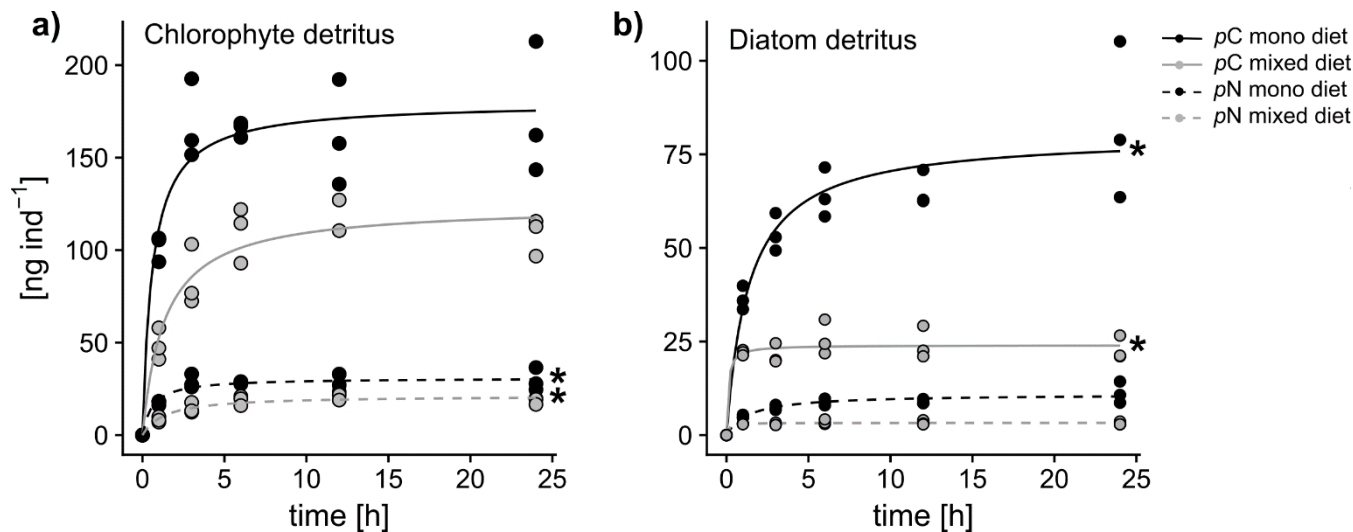
620 Figure 3 a-b. Comparison of chlorophyte and diatom phytodetritus feeding in A. tepida for 24 hours, presenting feeding dynamics for a) chlorophyte detritus and b) diatom detritus. Curves show Michaelis Menten Fits through triplicates for each approach (stars indicate calculated values for pC or pN).
