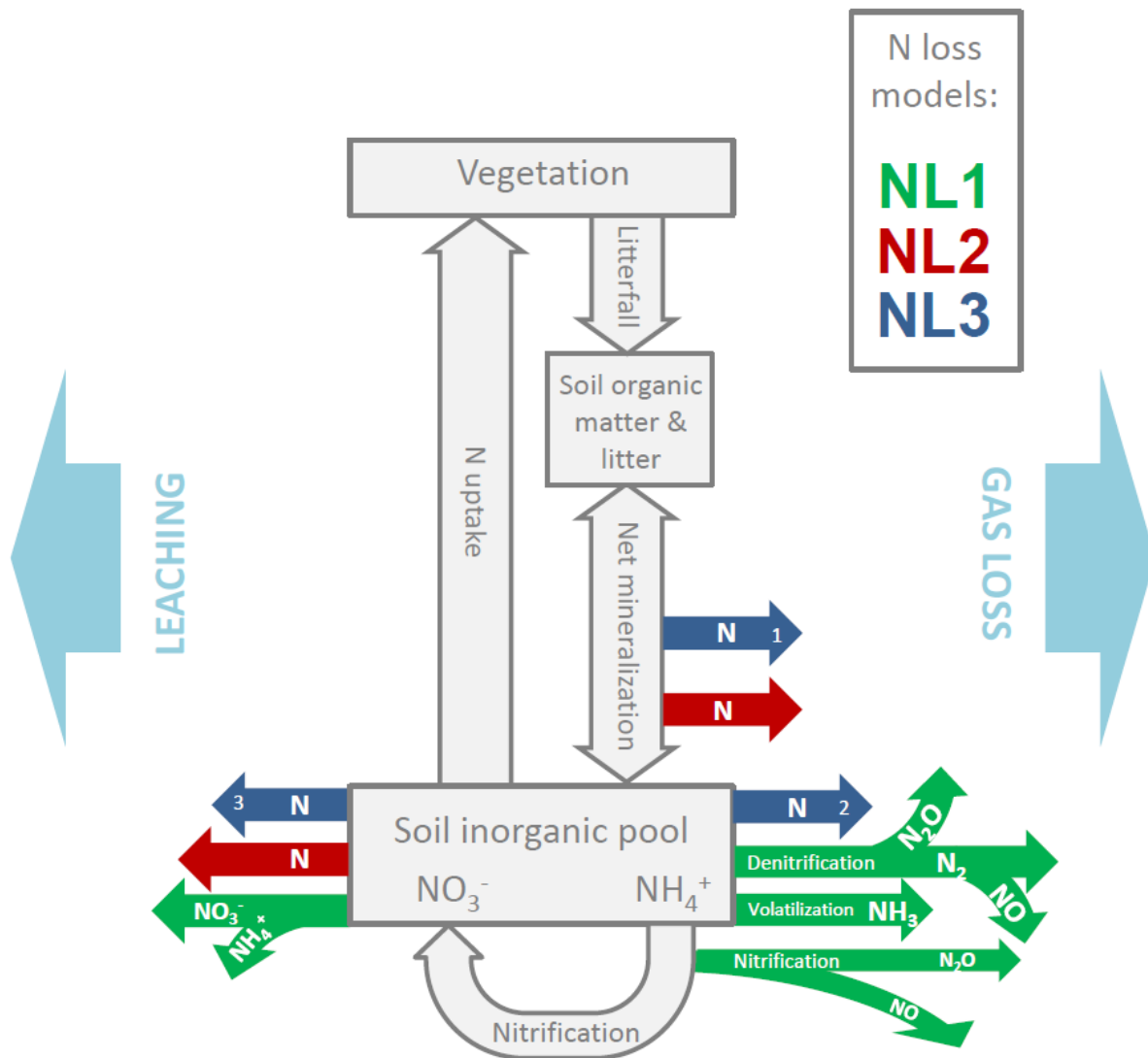
5 Figure 1: Simplified representation of the modelled internal nitrogen (N) cycle and the three employed N loss algorithms. External input fluxes from deposition and biological fixation are not shown. Grey boxes and arrows indicate N pools (vegetation, soil organic matter, litter, soil inorganic pools) and fluxes (litterfall, net 10 mineralization, nitrification, uptake). Coloured arrows indicate N loss fluxes as they are calculated from different pool sizes and flux magnitudes according to the three algorithms NL1, NL2, and NL3. Numbers in the blue arrows indicate the sequential nature of the NL3 approach. N = generic nitrogen species, N 2 = dinitrogen; NO = nitric oxide; N 2 O = nitrous oxide; NH 3 = ammonia; NO 3 - = nitrate; NH 4 + = ammonium. Arrow orientation to the left/right indicates leaching/gaseous loss.
