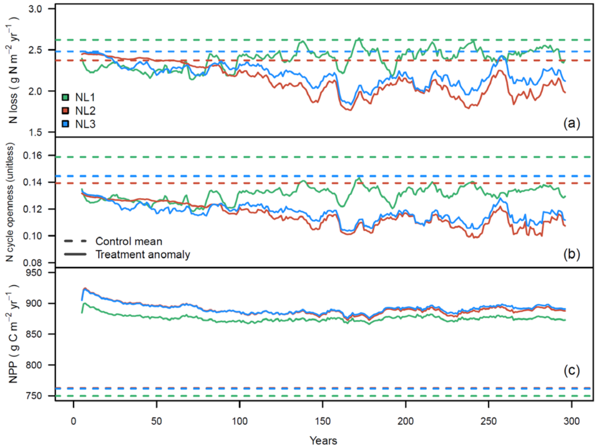
5 Figure 3: Ten year moving average responses of total nitrogen (N) loss (a; \text{g N m}^{-2} \text{ yr}^{-1} ), N cycle openness (N loss/net N mineralization; b; unitless) and net primary productivity (NPP; c; \text{g C m}^{-2} \text{ yr}^{-1} ) during the local 300 year \text{eCO}_2 simulation (380 ppm control + 200 ppm treatment) at the temperate "S 0 " site using the three N loss models. 300 year mean from the control runs and anomaly (treatment - control + control mean) from treatment simulations.
