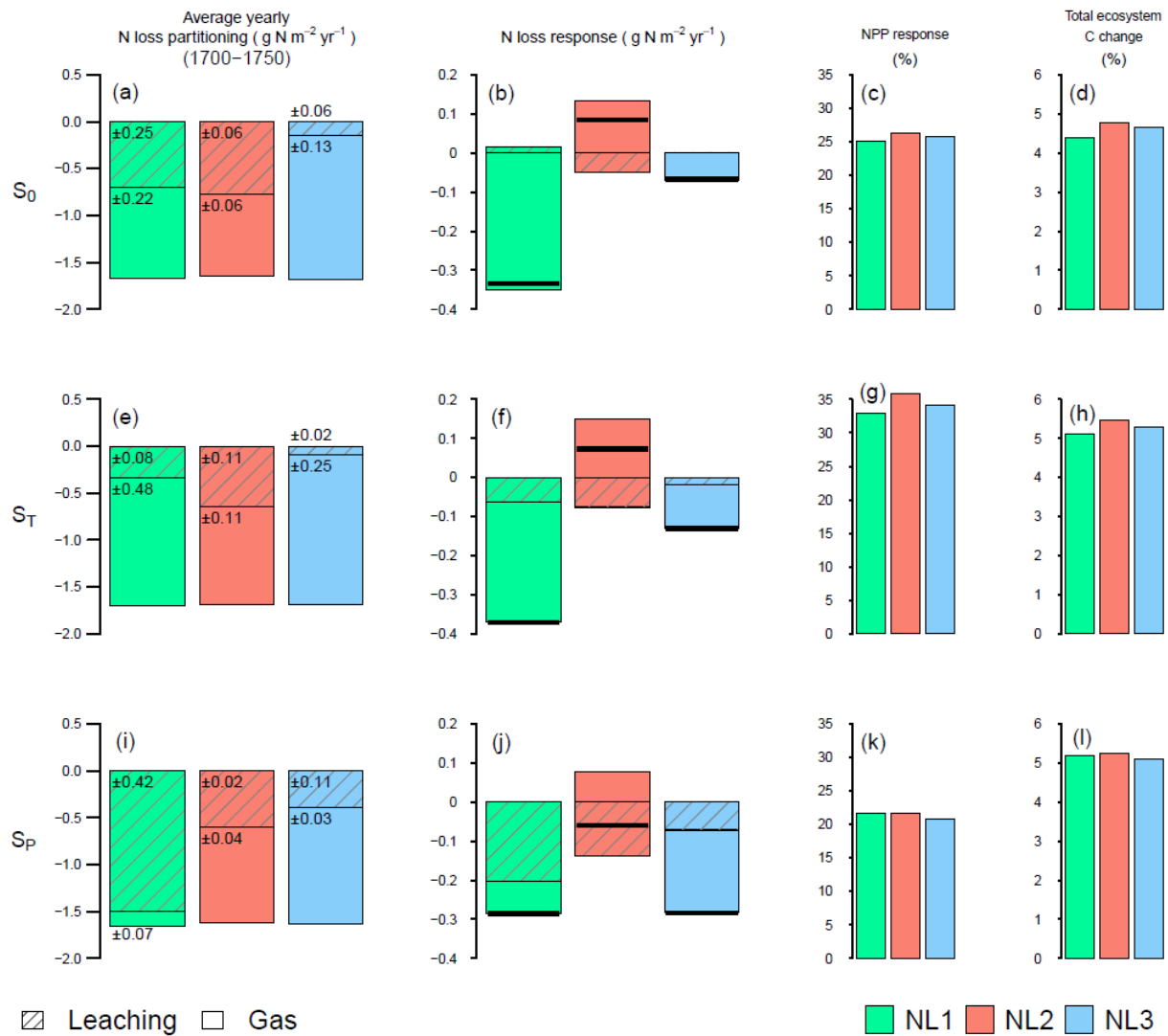
5 Figure 2: Average fate of ecosystem nitrogen (N) input at the three pseudosites " S_0 ", " S_T ", and " S_P " for the 1700-1750 quasi-equilibrium simulation period without perturbation (a, e, i; \text{g N m}^{-2} \text{yr}^{-1} ). Average N loss rate responses ( \text{g N m}^{-2} \text{yr}^{-1} ) to ten years of simulated elevated atmospheric \text{CO}_2 ( \text{eCO}_2 , +200 ppm) (b, f, j). Net primary productivity (NPP) responses (%) after ten years of \text{eCO}_2 , relative to control simulations (c, g, k). Change (%) of total ecosystem carbon (C) after ten years of \text{eCO}_2 , relative to the start of the experiment (d, h, l). Colours indicate the applied N loss algorithm (NL1, NL2, NL3). For a, b, e, f, i, and j, shading lines indicate leaching, unshaded colour indicates gaseous loss. Numbers on the bars indicate the standard deviation ( \text{g N m}^{-2} \text{yr}^{-1} ) of the leaching and gas loss components over the 1700-1750 quasi-equilibrium period. For a, e, and i, the sums of N allocation to organic pools (vegetation biomass and soil organic matter) were in the range of -0.07 - 0.01 \text{g N m}^{-2} \text{yr}^{-1} and were omitted here. External inputs of reactive N (biological N fixation + N deposition) were fixed at 1.631 \text{g N m}^{-2} \text{yr}^{-1} . For b, f, and j, black bars indicate the total N loss responses (gaseous loss + leaching). 10 15
